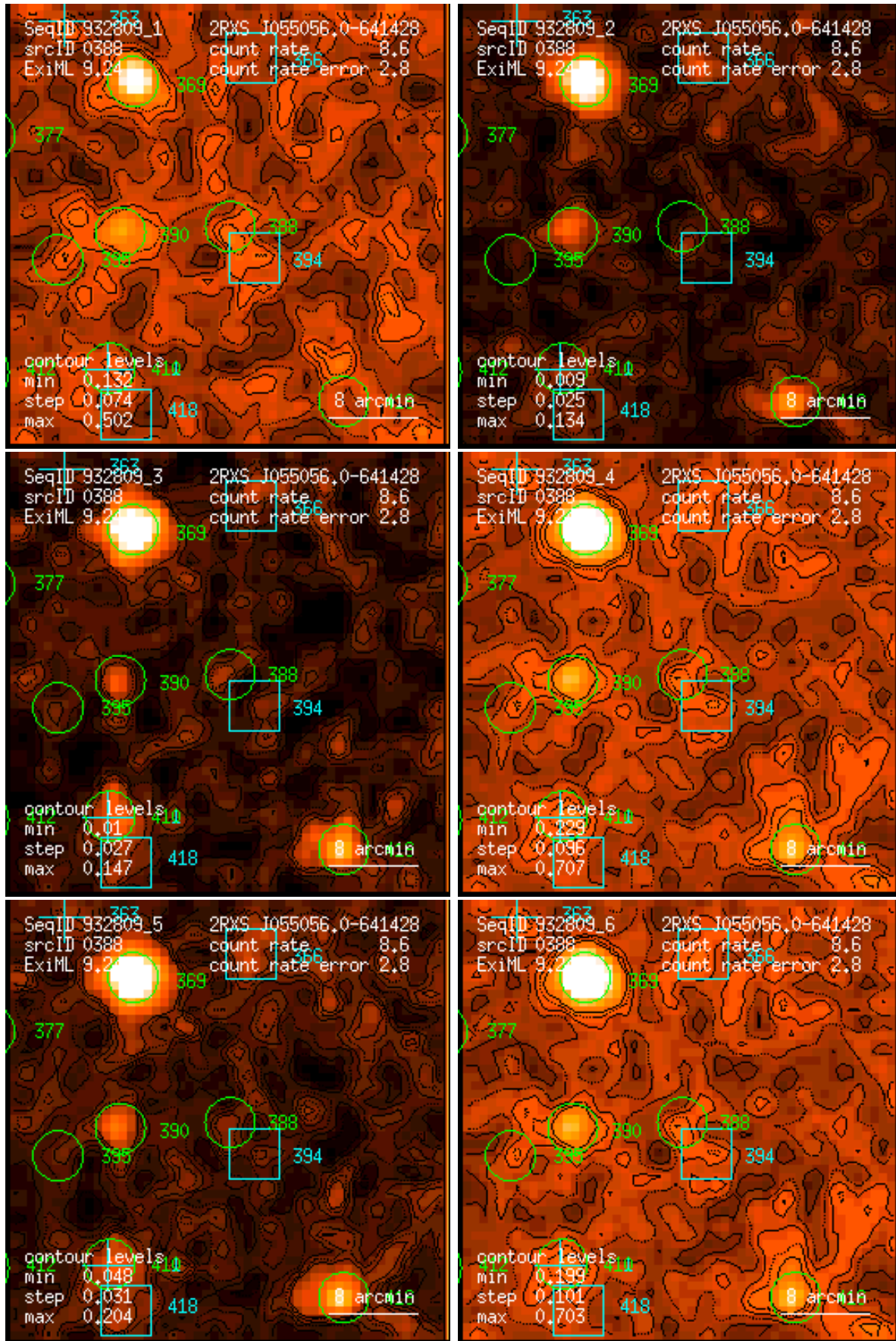
Figure 388: RASS 932809: detection 0388: band rate images, Gaussian filter: (1) PSPC channels 11 – 41, (2) 52 – 90, (3) 91 – 201, (4) 11 – 235, (5) 52 – 201, (6) 11 – 201. Broad band rates in counts/ks. Band rate contour levels in counts/ks/arcmin 2 .
