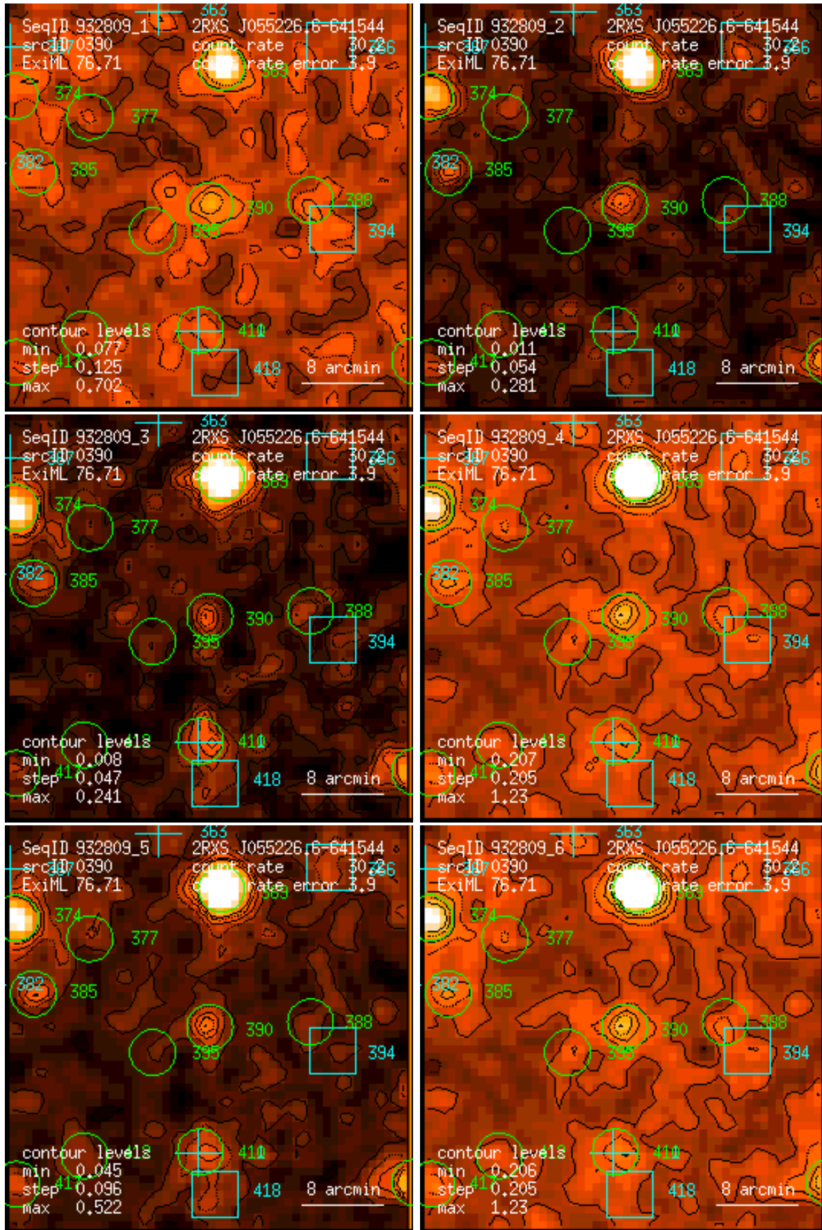
Figure 390: RASS 932809: detection 0390: band rate images, Gaussian filter: (1) PSPC channels 11 – 41, (2) 52 – 90, (3) 91 – 201, (4) 11 – 235, (5) 52 – 201, (6) 11 – 201. Broad band rates in counts/ks. Band rate contour levels in counts/ks/arcmin 2 .
