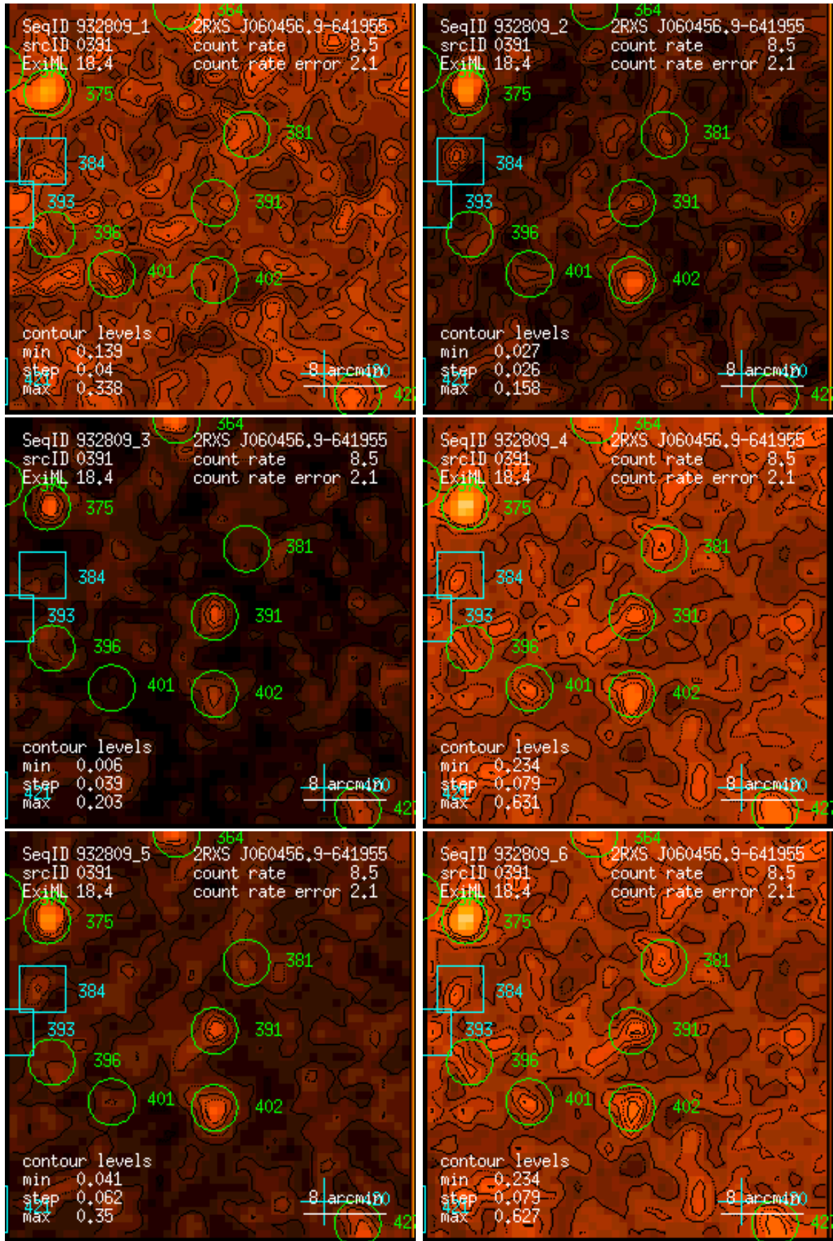
Figure 391: RASS 932809: detection 0391: band rate images, Gaussian filter: (1) PSPC channels 11 – 41, (2) 52 – 90, (3) 91 – 201, (4) 11 – 235, (5) 52 – 201, (6) 11 – 201. Broad band rates in counts/ks. Band rate contour levels in counts/ks/arcmin 2 .
