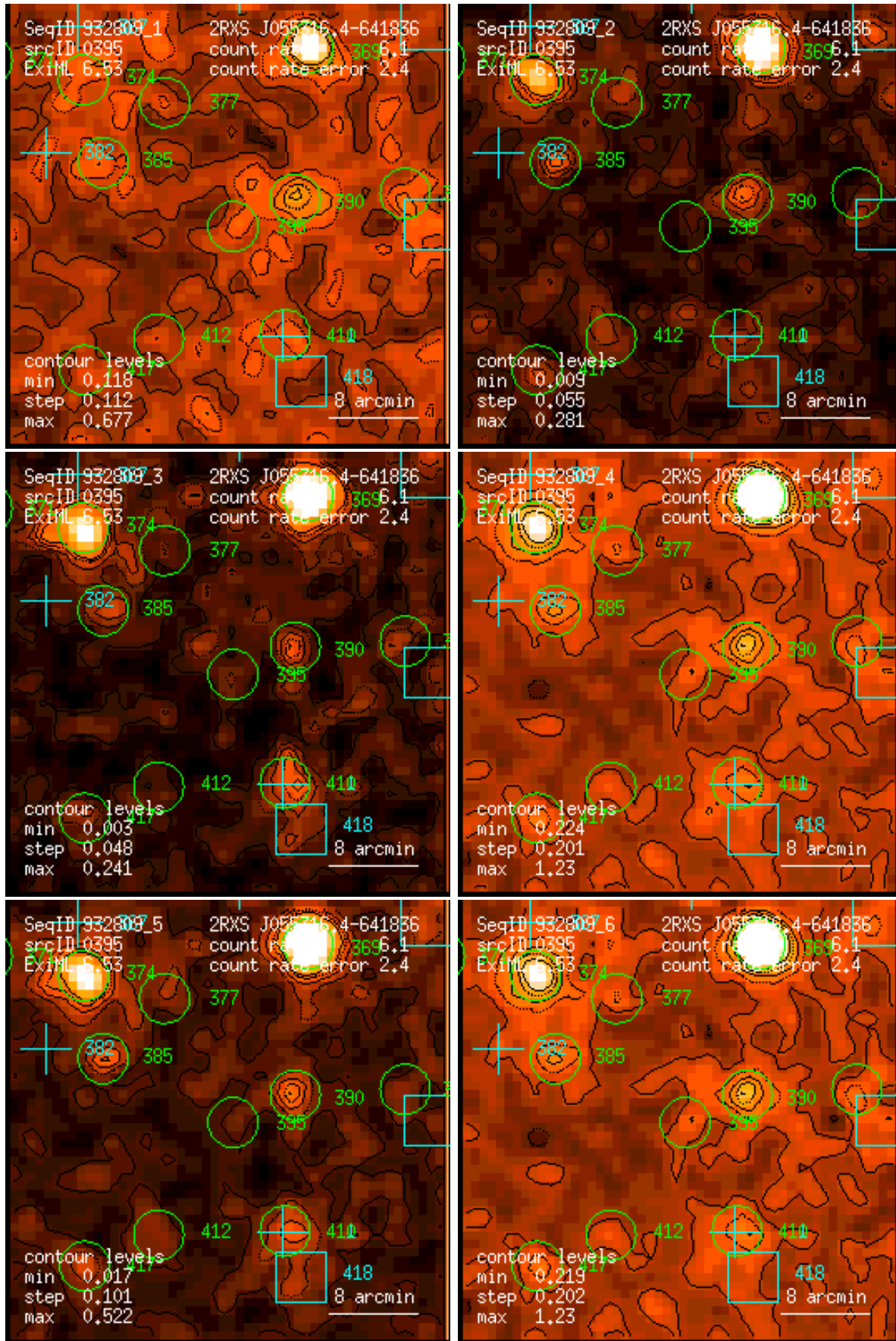
Figure 395: RASS 932809: detection 0395: band rate images, Gaussian filter: (1) PSPC channels 11 – 41, (2) 52 – 90, (3) 91 – 201, (4) 11 – 235, (5) 52 – 201, (6) 11 – 201. Broad band rates in counts/ks. Band rate contour levels in counts/ks/arcmin 2 .
