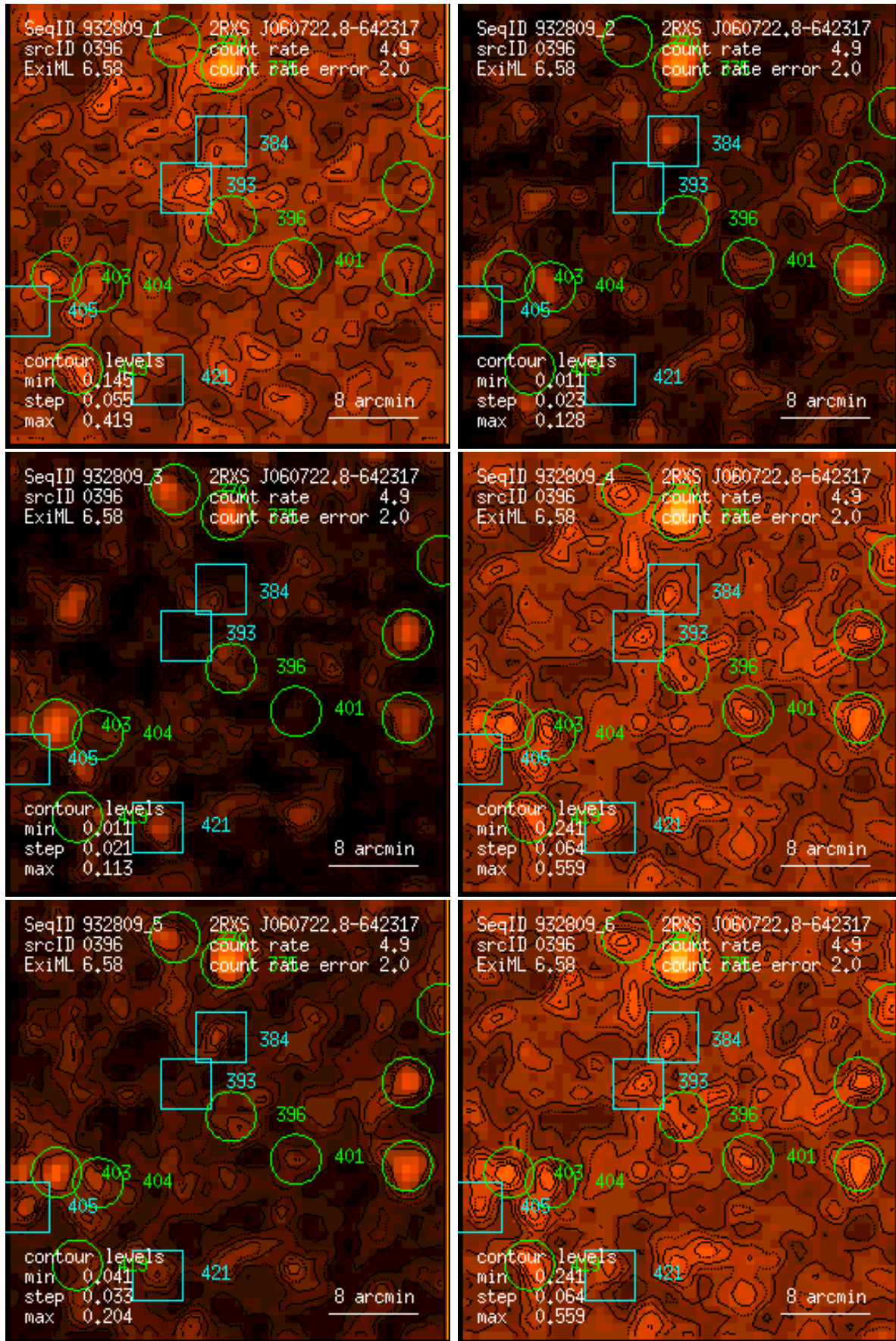
Figure 396: RASS 932809: detection 0396: band rate images, Gaussian filter: (1) PSPC channels 11 – 41, (2) 52 – 90, (3) 91 – 201, (4) 11 – 235, (5) 52 – 201, (6) 11 – 201. Broad band rates in counts/ks. Band rate contour levels in counts/ks/arcmin 2 .
