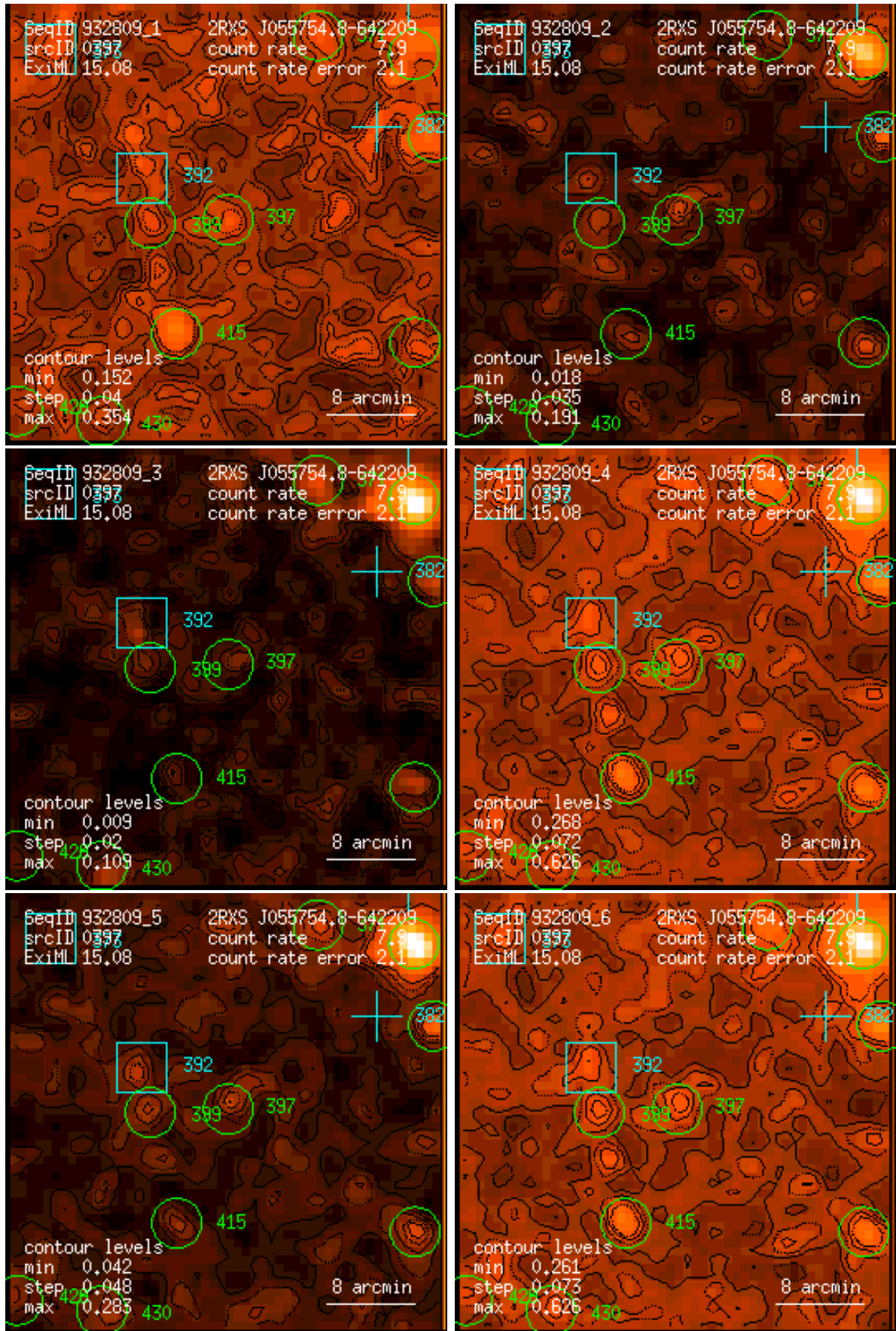
Figure 397: RASS 932809: detection 0397: band rate images, Gaussian filter: (1) PSPC channels 11 – 41, (2) 52 – 90, (3) 91 – 201, (4) 11 – 235, (5) 52 – 201, (6) 11 – 201. Broad band rates in counts/ks. Band rate contour levels in counts/ks/arcmin 2 .
