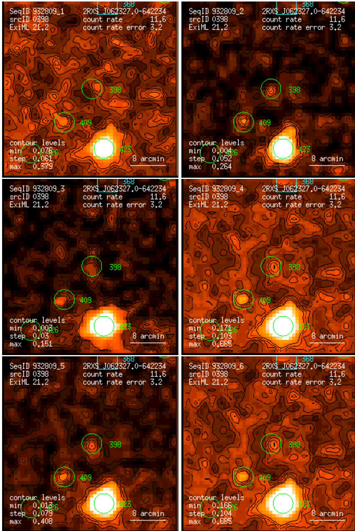
Figure 398: RASS 932809: detection 0398: band rate images, Gaussian filter: (1) PSPC channels 11 – 41, (2) 52 – 90, (3) 91 – 201, (4) 11 – 235, (5) 52 – 201, (6) 11 – 201. Broad band rates in counts/ks. Band rate contour levels in counts/ks/arcmin 2 .
