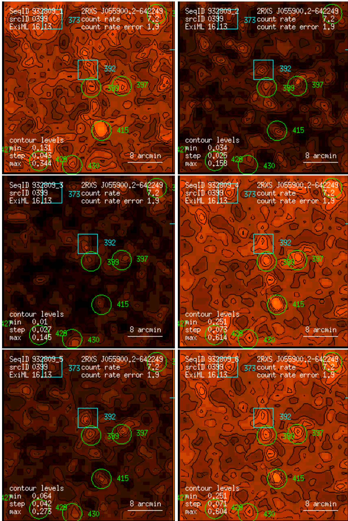
Figure 399: RASS 932809: detection 0399: band rate images, Gaussian filter: (1) PSPC channels 11 – 41, (2) 52 – 90, (3) 91 – 201, (4) 11 – 235, (5) 52 – 201, (6) 11 – 201. Broad band rates in counts/ks. Band rate contour levels in counts/ks/arcmin 2 .
