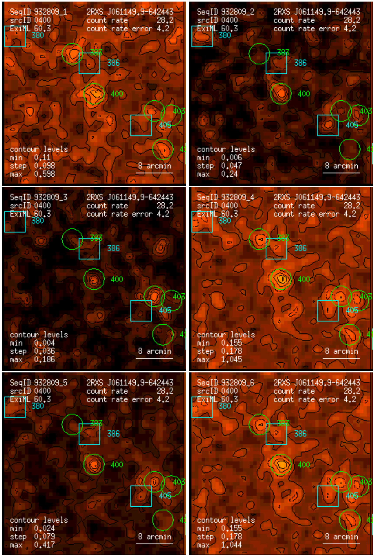
Figure 400: RASS 932809: detection 0400: band rate images, Gaussian filter: (1) PSPC channels 11 – 41, (2) 52 – 90, (3) 91 – 201, (4) 11 – 235, (5) 52 – 201, (6) 11 – 201. Broad band rates in counts/ks. Band rate contour levels in counts/ks/arcmin 2 .
