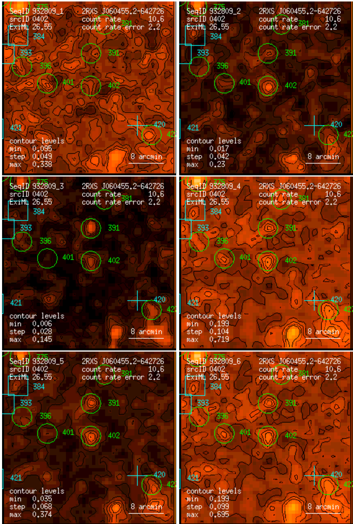
Figure 402: RASS 932809: detection 0402: band rate images, Gaussian filter: (1) PSPC channels 11 – 41, (2) 52 – 90, (3) 91 – 201, (4) 11 – 235, (5) 52 – 201, (6) 11 – 201. Broad band rates in counts/ks. Band rate contour levels in counts/ks/arcmin 2 .
