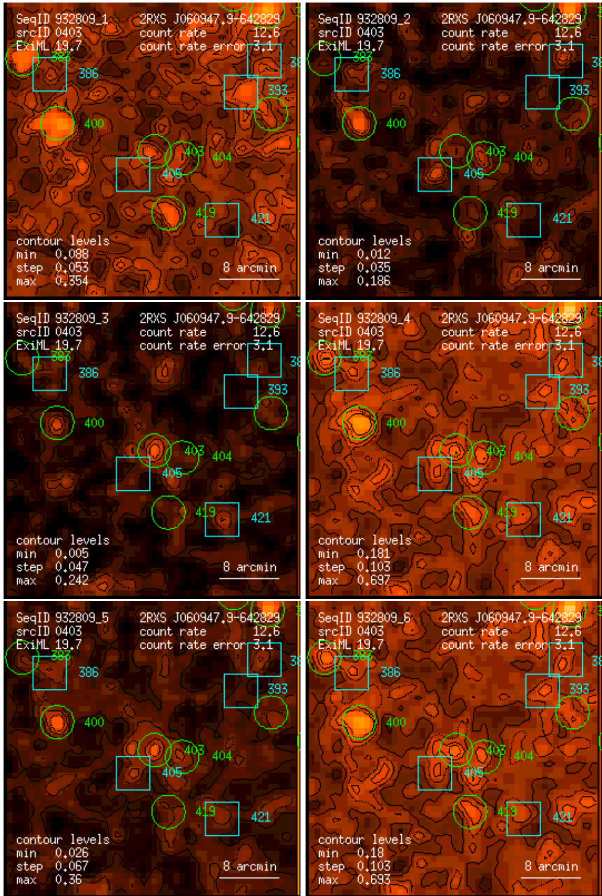
Figure 403: RASS 932809: detection 0403: band rate images, Gaussian filter: (1) PSPC channels 11 – 41, (2) 52 – 90, (3) 91 – 201, (4) 11 – 235, (5) 52 – 201, (6) 11 – 201. Broad band rates in counts/ks. Band rate contour levels in counts/ks/arcmin 2 .
