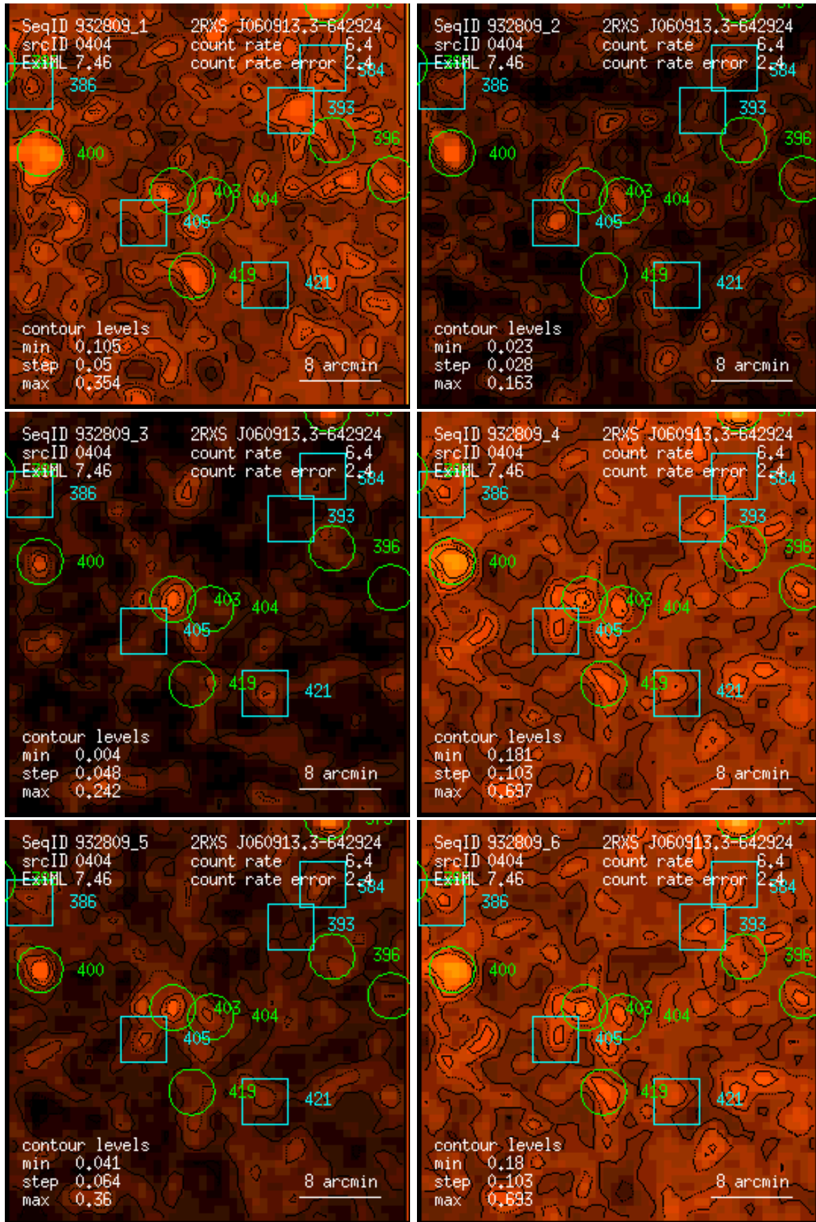
Figure 404: RASS 932809: detection 0404: band rate images, Gaussian filter: (1) PSPC channels 11 – 41, (2) 52 – 90, (3) 91 – 201, (4) 11 – 235, (5) 52 – 201, (6) 11 – 201. Broad band rates in counts/ks. Band rate contour levels in counts/ks/arcmin 2 .
