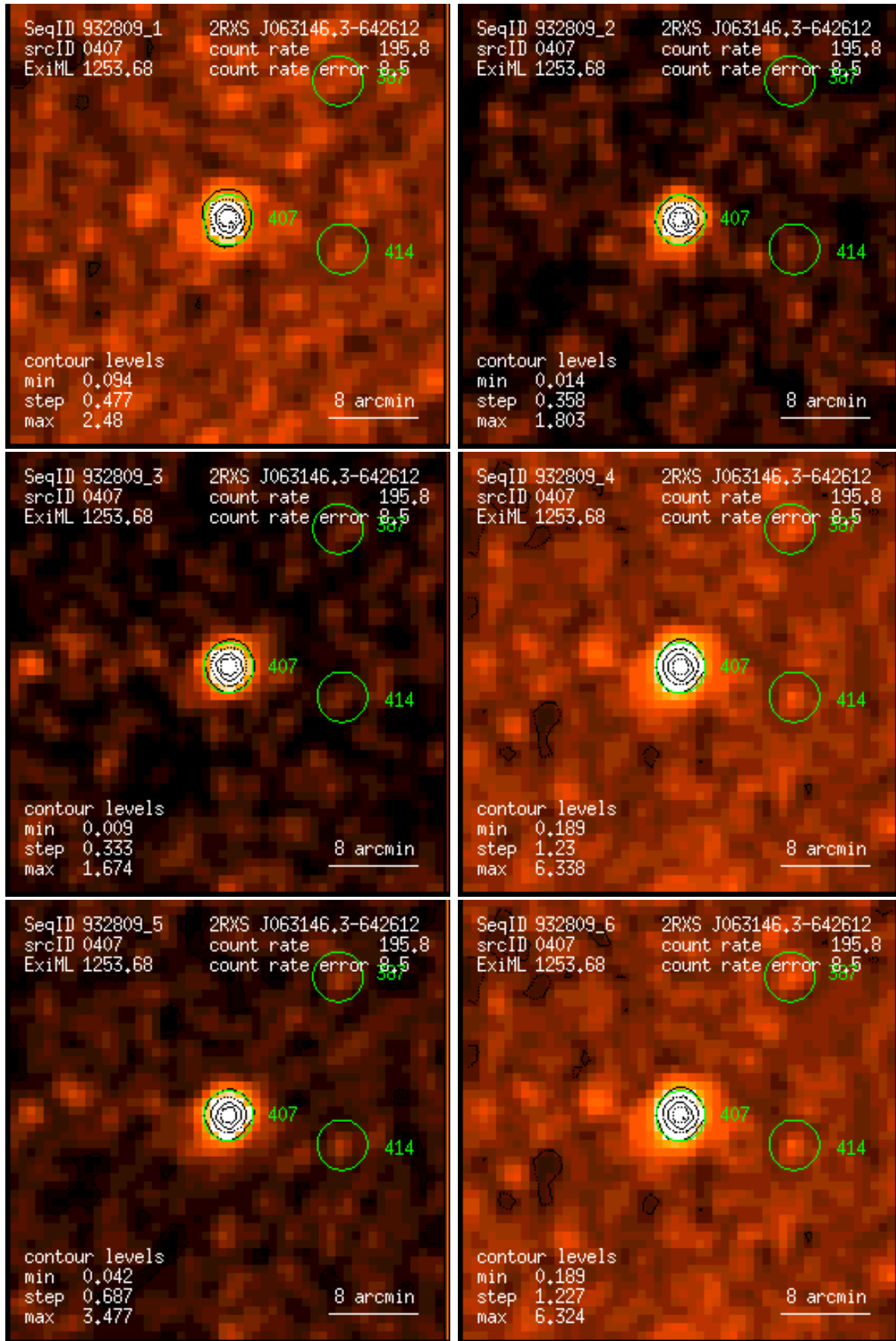
Figure 407: RASS 932809: detection 0407: band rate images, Gaussian filter: (1) PSPC channels 11 – 41, (2) 52 – 90, (3) 91 – 201, (4) 11 – 235, (5) 52 – 201, (6) 11 – 201. Broad band rates in counts/ks. Band rate contour levels in counts/ks/arcmin 2 .
