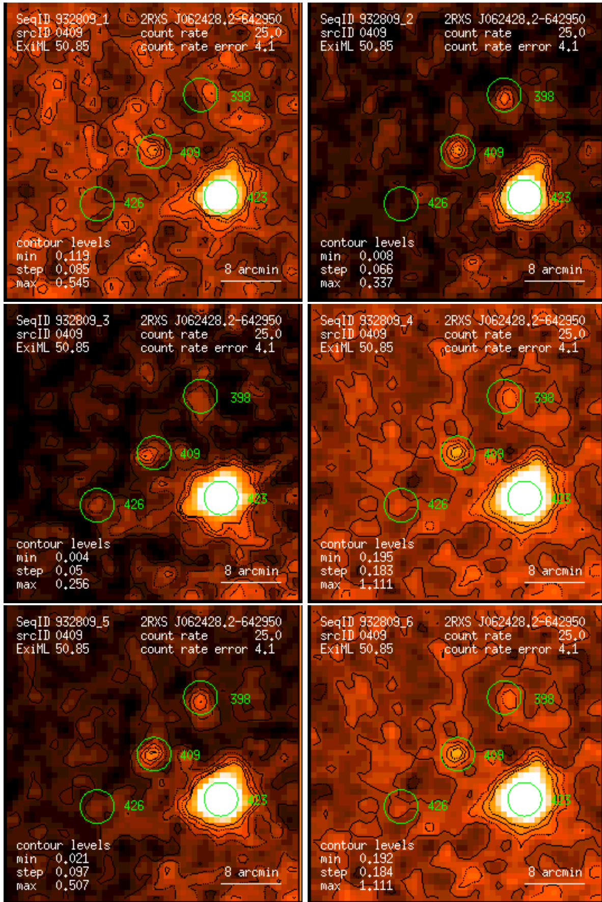
Figure 409: RASS 932809: detection 0409: band rate images, Gaussian filter: (1) PSPC channels 11 – 41, (2) 52 – 90, (3) 91 – 201, (4) 11 – 235, (5) 52 – 201, (6) 11 – 201. Broad band rates in counts/ks. Band rate contour levels in counts/ks/arcmin 2 .
