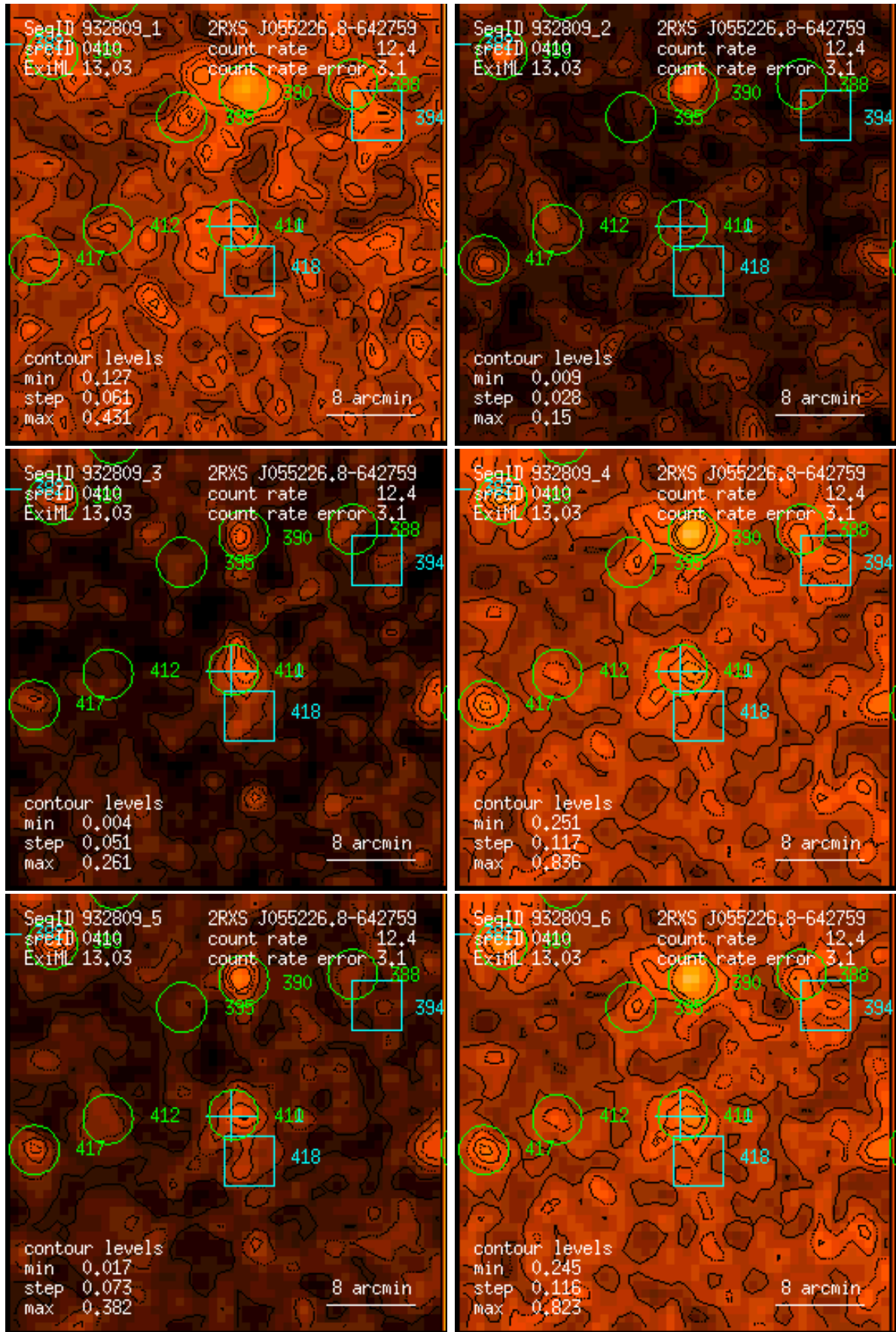
Figure 410: RASS 932809: detection 0410: band rate images, Gaussian filter: (1) PSPC channels 11 – 41, (2) 52 – 90, (3) 91 – 201, (4) 11 – 235, (5) 52 – 201, (6) 11 – 201. Broad band rates in counts/ks. Band rate contour levels in counts/ks/arcmin 2 .
