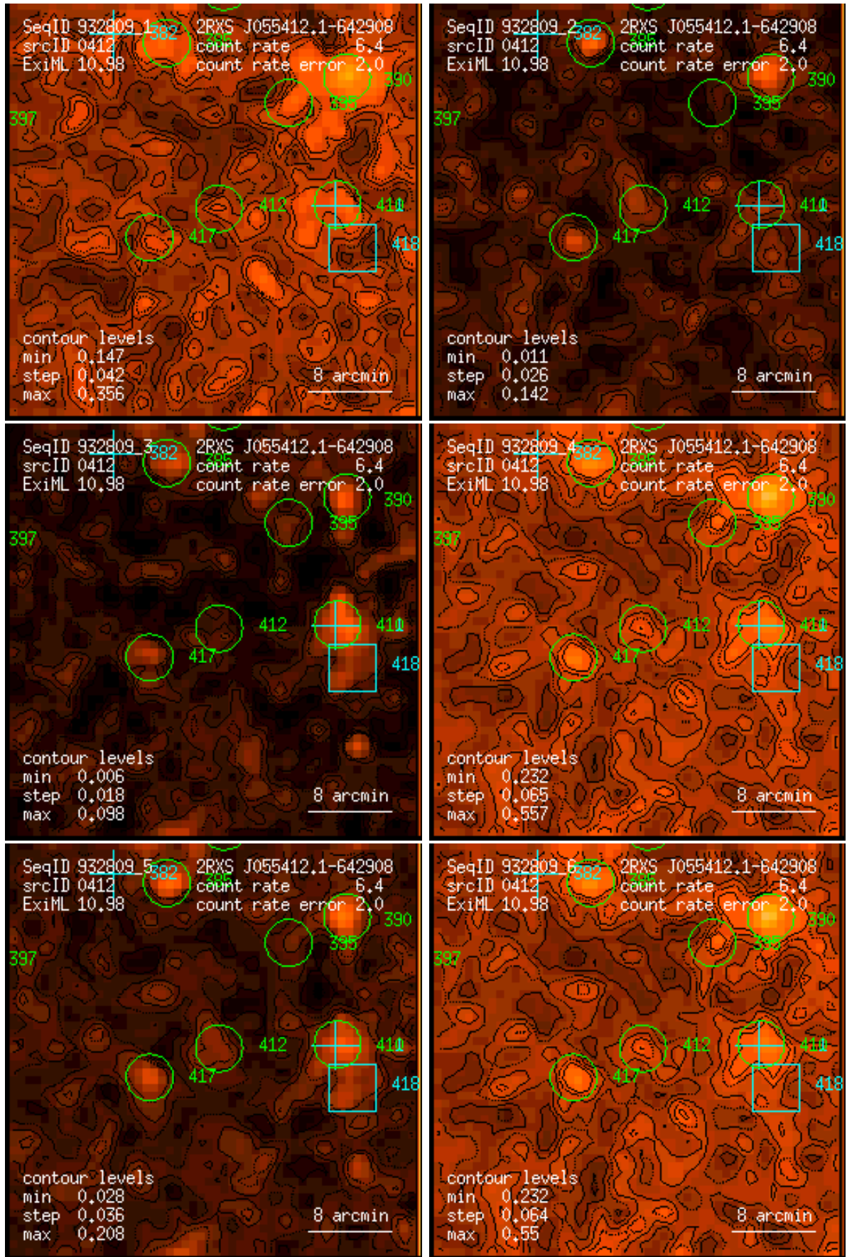
Figure 412: RASS 932809: detection 0412: band rate images, Gaussian filter: (1) PSPC channels 11 – 41, (2) 52 – 90, (3) 91 – 201, (4) 11 – 235, (5) 52 – 201, (6) 11 – 201. Broad band rates in counts/ks. Band rate contour levels in counts/ks/arcmin 2 .
