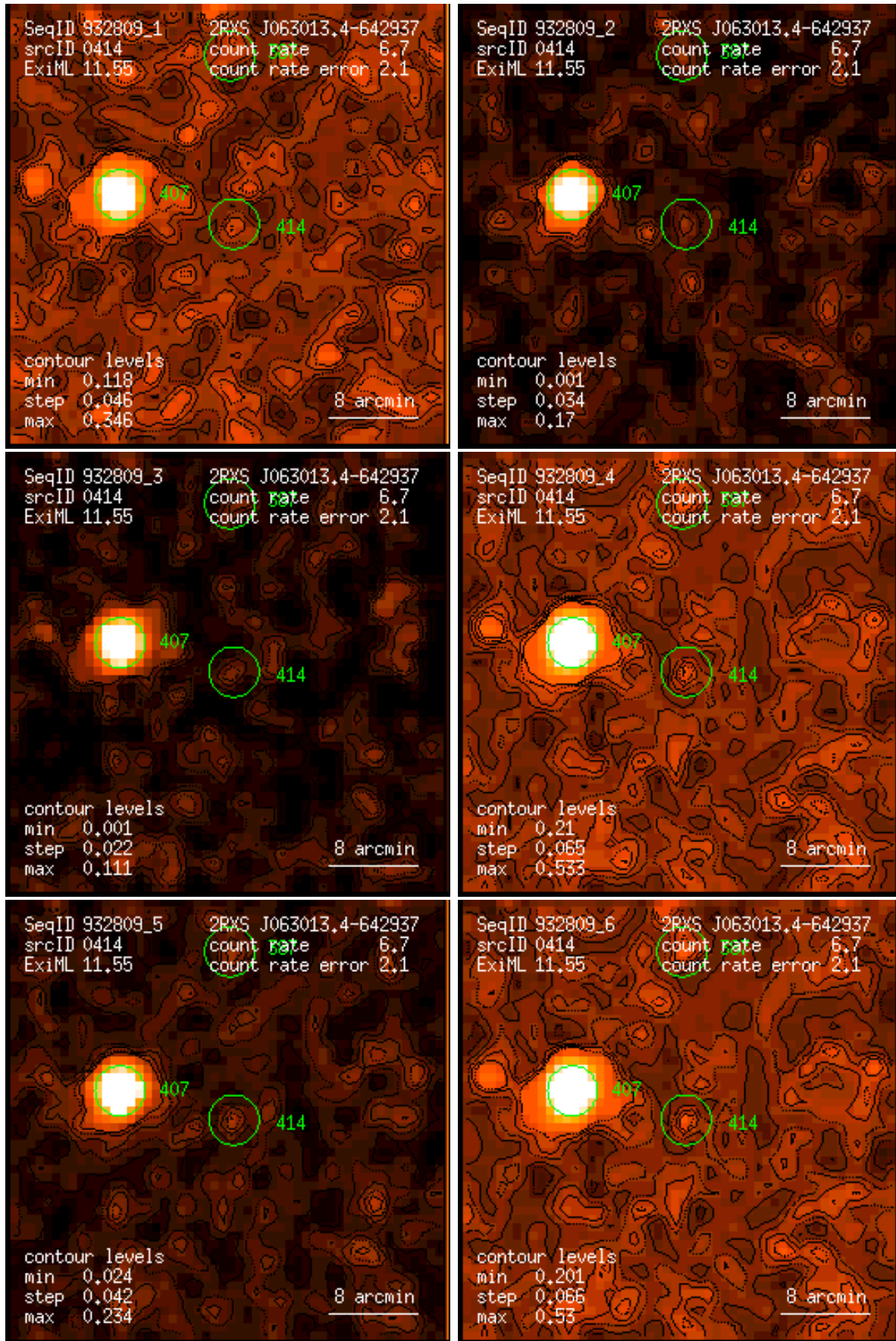
Figure 414: RASS 932809: detection 0414: band rate images, Gaussian filter: (1) PSPC channels 11 – 41, (2) 52 – 90, (3) 91 – 201, (4) 11 – 235, (5) 52 – 201, (6) 11 – 201. Broad band rates in counts/ks. Band rate contour levels in counts/ks/arcmin 2 .
