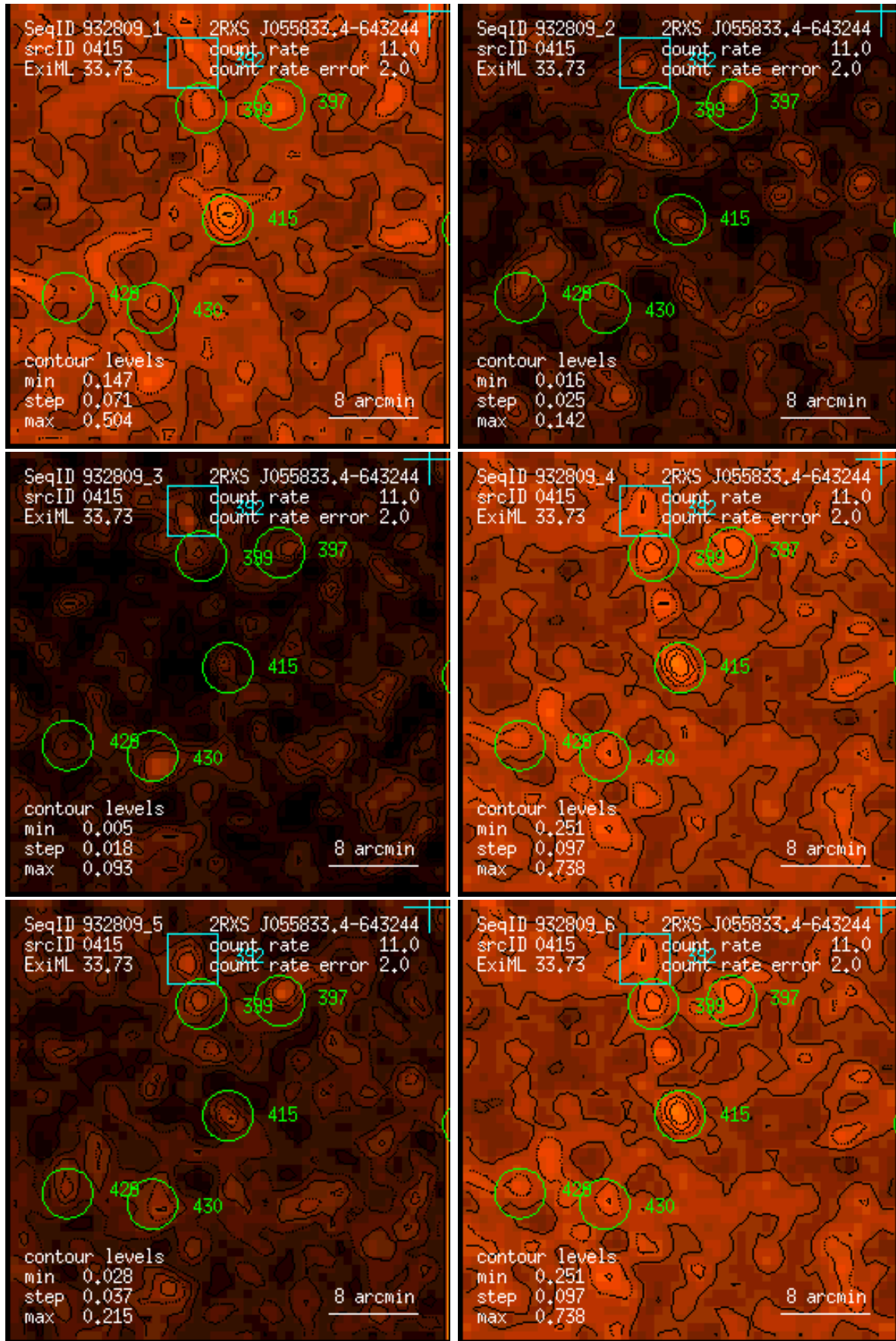
Figure 415: RASS 932809: detection 0415: band rate images, Gaussian filter: (1) PSPC channels 11 – 41, (2) 52 – 90, (3) 91 – 201, (4) 11 – 235, (5) 52 – 201, (6) 11 – 201. Broad band rates in counts/ks. Band rate contour levels in counts/ks/arcmin 2 .
