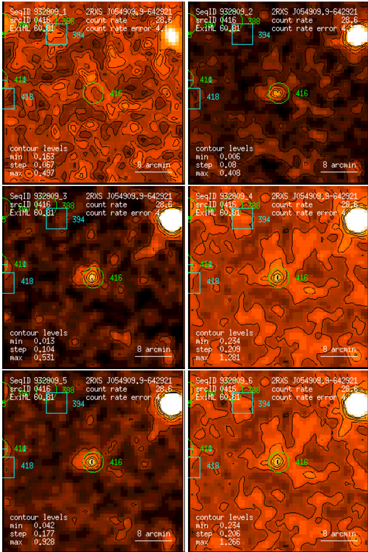
Figure 416: RASS 932809: detection 0416: band rate images, Gaussian filter: (1) PSPC channels 11 – 41, (2) 52 – 90, (3) 91 – 201, (4) 11 – 235, (5) 52 – 201, (6) 11 – 201. Broad band rates in counts/ks. Band rate contour levels in counts/ks/arcmin 2 .
