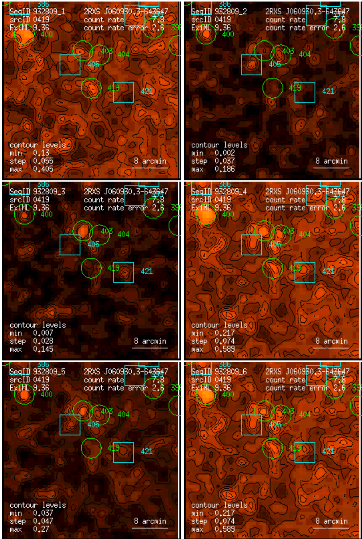
Figure 419: RASS 932809: detection 0419: band rate images, Gaussian filter: (1) PSPC channels 11 – 41, (2) 52 – 90, (3) 91 – 201, (4) 11 – 235, (5) 52 – 201, (6) 11 – 201. Broad band rates in counts/ks. Band rate contour levels in counts/ks/arcmin 2 .
