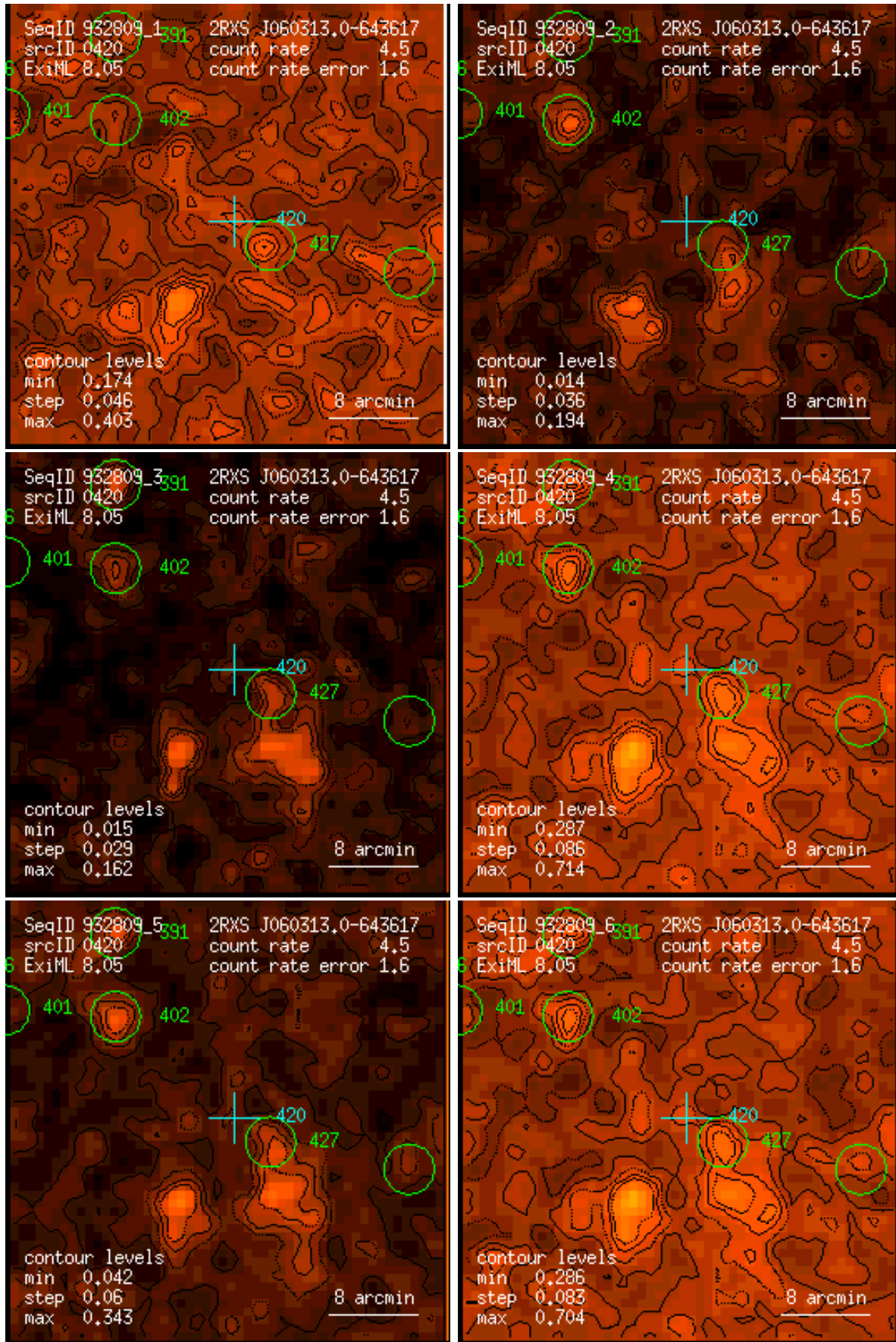
Figure 420: RASS 932809: detection 0420: band rate images, Gaussian filter: (1) PSPC channels 11 – 41, (2) 52 – 90, (3) 91 – 201, (4) 11 – 235, (5) 52 – 201, (6) 11 – 201. Broad band rates in counts/ks. Band rate contour levels in counts/ks/arcmin 2 .
