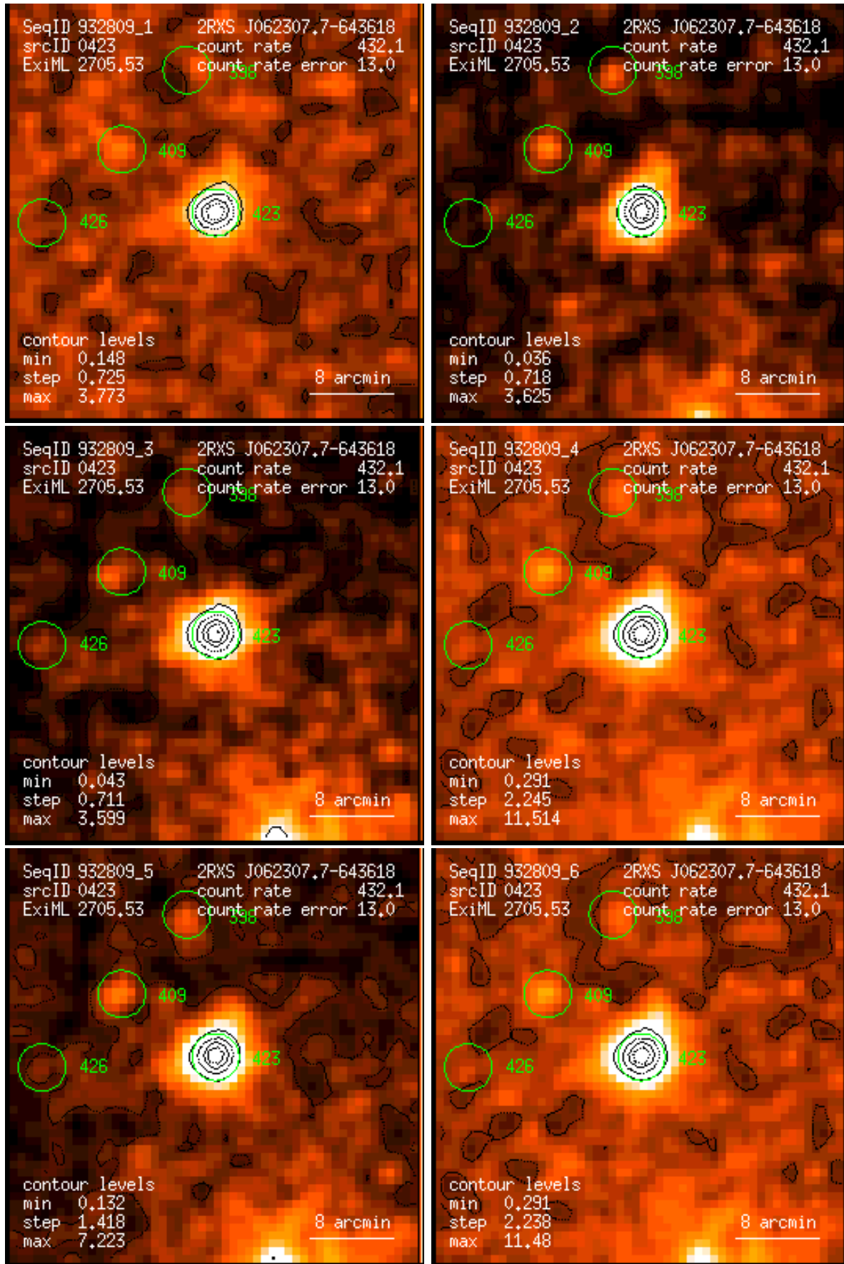
Figure 423: RASS 932809: detection 0423: band rate images, Gaussian filter: (1) PSPC channels 11 – 41, (2) 52 – 90, (3) 91 – 201, (4) 11 – 235, (5) 52 – 201, (6) 11 – 201. Broad band rates in counts/ks. Band rate contour levels in counts/ks/arcmin 2 .
