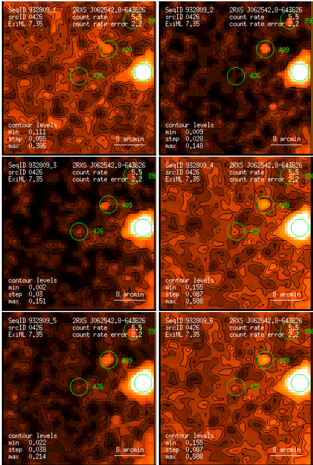
Figure 426: RASS 932809: detection 0426: band rate images, Gaussian filter: (1) PSPC channels 11 – 41, (2) 52 – 90, (3) 91 – 201, (4) 11 – 235, (5) 52 – 201, (6) 11 – 201. Broad band rates in counts/ks. Band rate contour levels in counts/ks/arcmin 2 .
