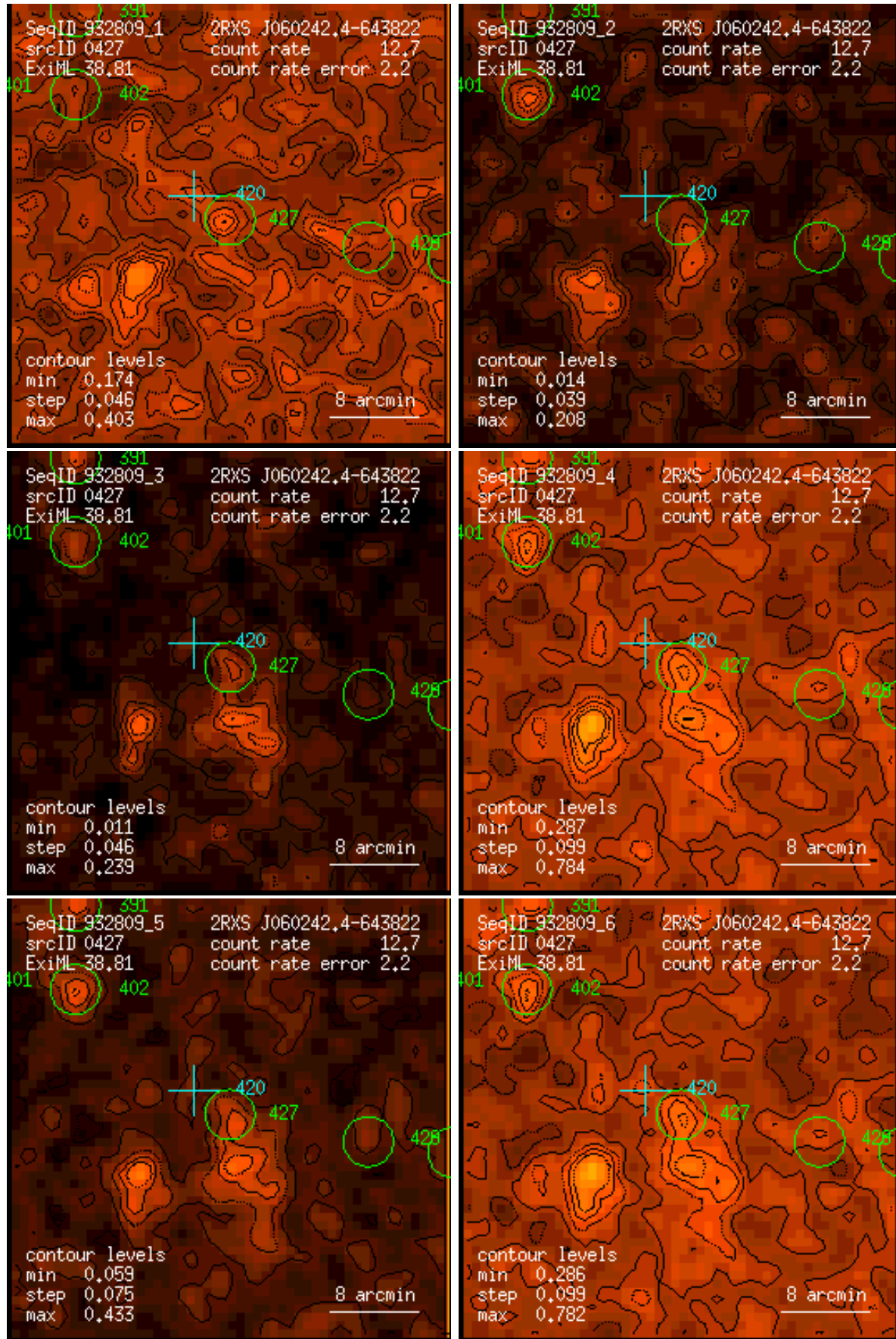
Figure 427: RASS 932809: detection 0427: band rate images, Gaussian filter: (1) PSPC channels 11 – 41, (2) 52 – 90, (3) 91 – 201, (4) 11 – 235, (5) 52 – 201, (6) 11 – 201. Broad band rates in counts/ks. Band rate contour levels in counts/ks/arcmin 2 .
