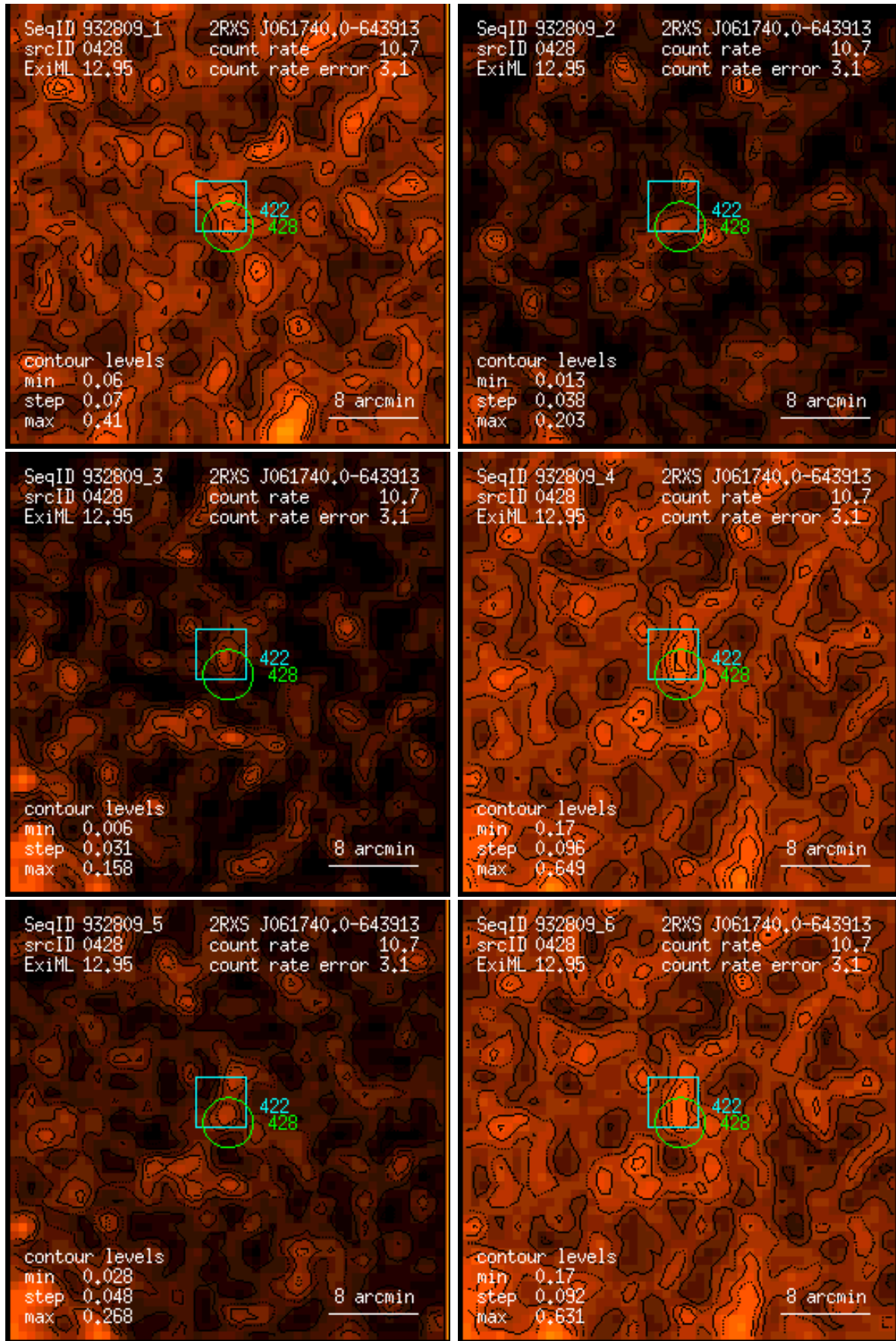
Figure 428: RASS 932809: detection 0428: band rate images, Gaussian filter: (1) PSPC channels 11 – 41, (2) 52 – 90, (3) 91 – 201, (4) 11 – 235, (5) 52 – 201, (6) 11 – 201. Broad band rates in counts/ks. Band rate contour levels in counts/ks/arcmin 2 .
