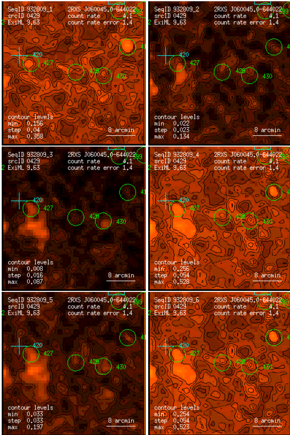
Figure 429: RASS 932809: detection 0429: band rate images, Gaussian filter: (1) PSPC channels 11 – 41, (2) 52 – 90, (3) 91 – 201, (4) 11 – 235, (5) 52 – 201, (6) 11 – 201. Broad band rates in counts/ks. Band rate contour levels in counts/ks/arcmin 2 .
