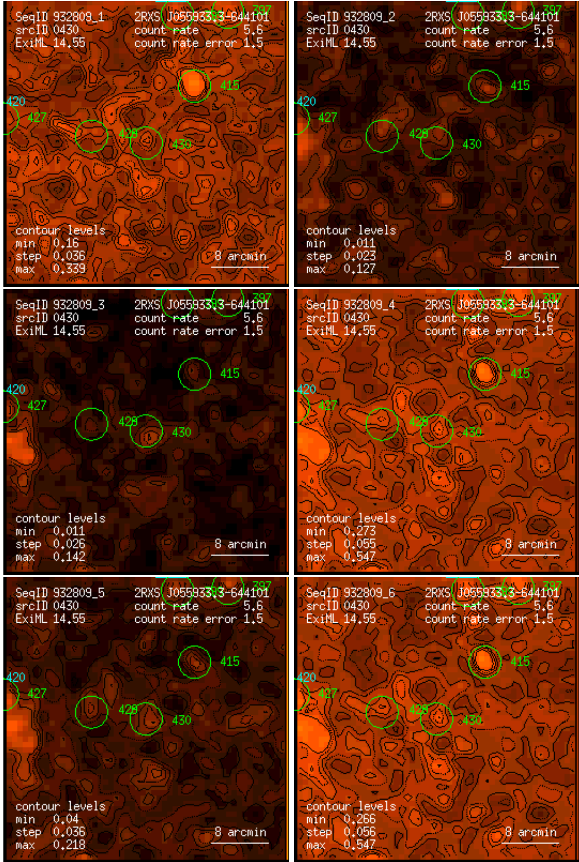
Figure 430: RASS 932809: detection 0430: band rate images, Gaussian filter: (1) PSPC channels 11 – 41, (2) 52 – 90, (3) 91 – 201, (4) 11 – 235, (5) 52 – 201, (6) 11 – 201. Broad band rates in counts/ks. Band rate contour levels in counts/ks/arcmin 2 .
