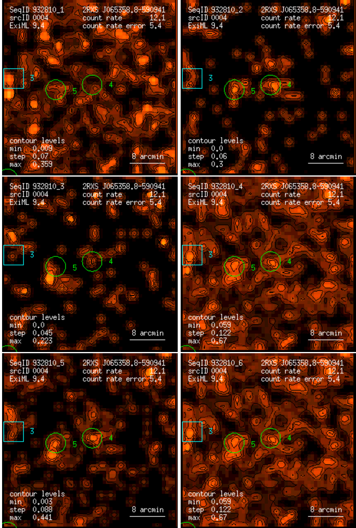
Figure 4: RASS 932810: detection 0004: band rate images, Gaussian filter: (1) PSPC channels 11 – 41, (2) 52 – 90, (3) 91 – 201, (4) 11 – 235, (5) 52 – 201, (6) 11 – 201. Broad band rates in counts/ks. Band rate contour levels in counts/ks/arcmin 2 .
