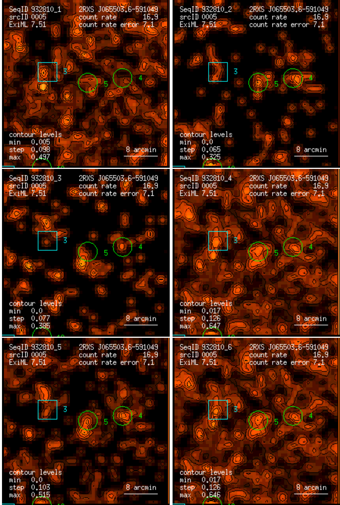
Figure 5: RASS 932810: detection 0005: band rate images, Gaussian filter: (1) PSPC channels 11 – 41, (2) 52 – 90, (3) 91 – 201, (4) 11 – 235, (5) 52 – 201, (6) 11 – 201. Broad band rates in counts/ks. Band rate contour levels in counts/ks/arcmin 2 .
