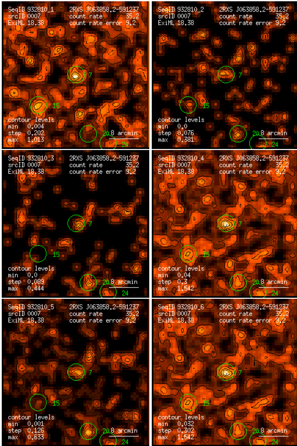
Figure 7: RASS 932810: detection 0007: band rate images, Gaussian filter: (1) PSPC channels 11 – 41, (2) 52 – 90, (3) 91 – 201, (4) 11 – 235, (5) 52 – 201, (6) 11 – 201. Broad band rates in counts/ks. Band rate contour levels in counts/ks/arcmin 2 .
