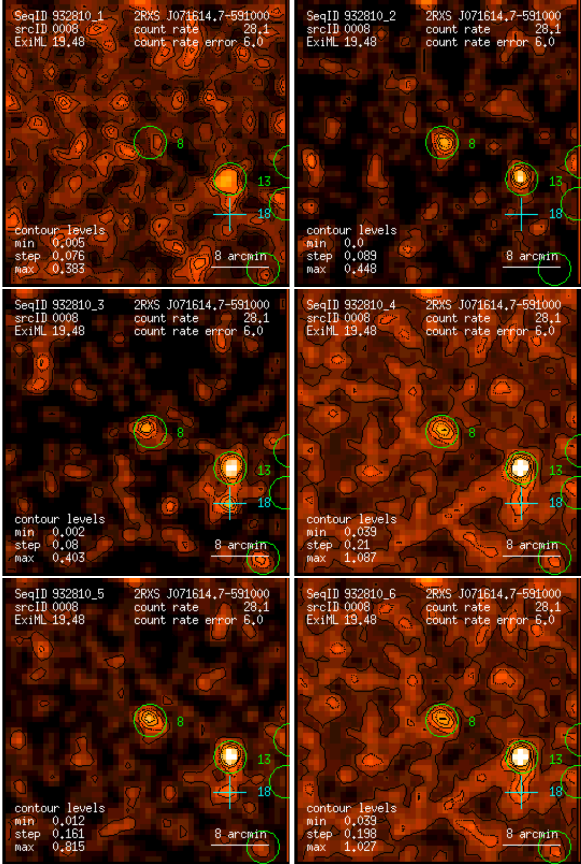
Figure 8: RASS 932810: detection 0008: band rate images, Gaussian filter: (1) PSPC channels 11 – 41, (2) 52 – 90, (3) 91 – 201, (4) 11 – 235, (5) 52 – 201, (6) 11 – 201. Broad band rates in counts/ks. Band rate contour levels in counts/ks/arcmin 2 .
