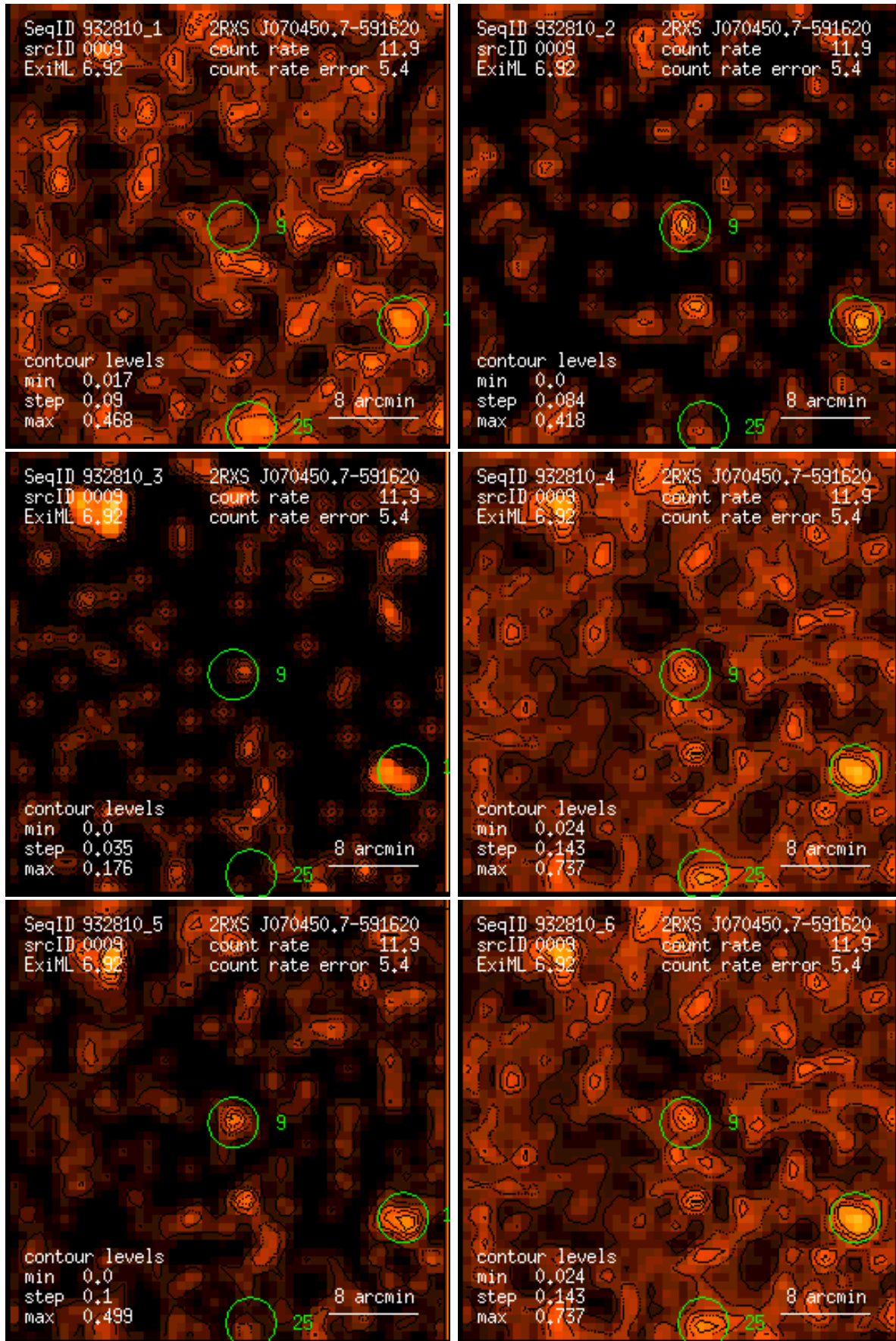
Figure 9: RASS 932810: detection 0009: band rate images, Gaussian filter: (1) PSPC channels 11 – 41, (2) 52 – 90, (3) 91 – 201, (4) 11 – 235, (5) 52 – 201, (6) 11 – 201. Broad band rates in counts/ks. Band rate contour levels in counts/ks/arcmin 2 .
