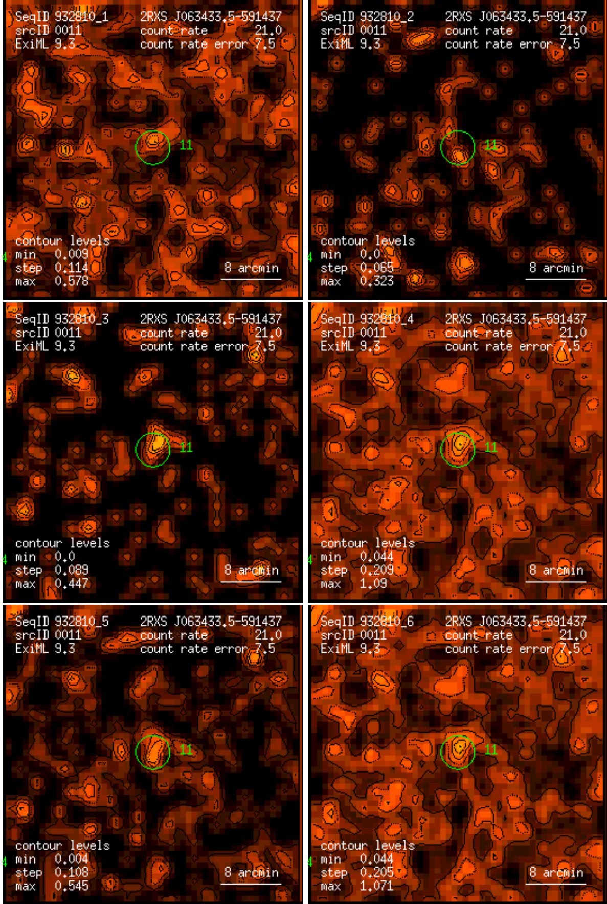
Figure 11: RASS 932810: detection 0011: band rate images, Gaussian filter: (1) PSPC channels 11 – 41, (2) 52 – 90, (3) 91 – 201, (4) 11 – 235, (5) 52 – 201, (6) 11 – 201. Broad band rates in counts/ks. Band rate contour levels in counts/ks/arcmin 2 .
