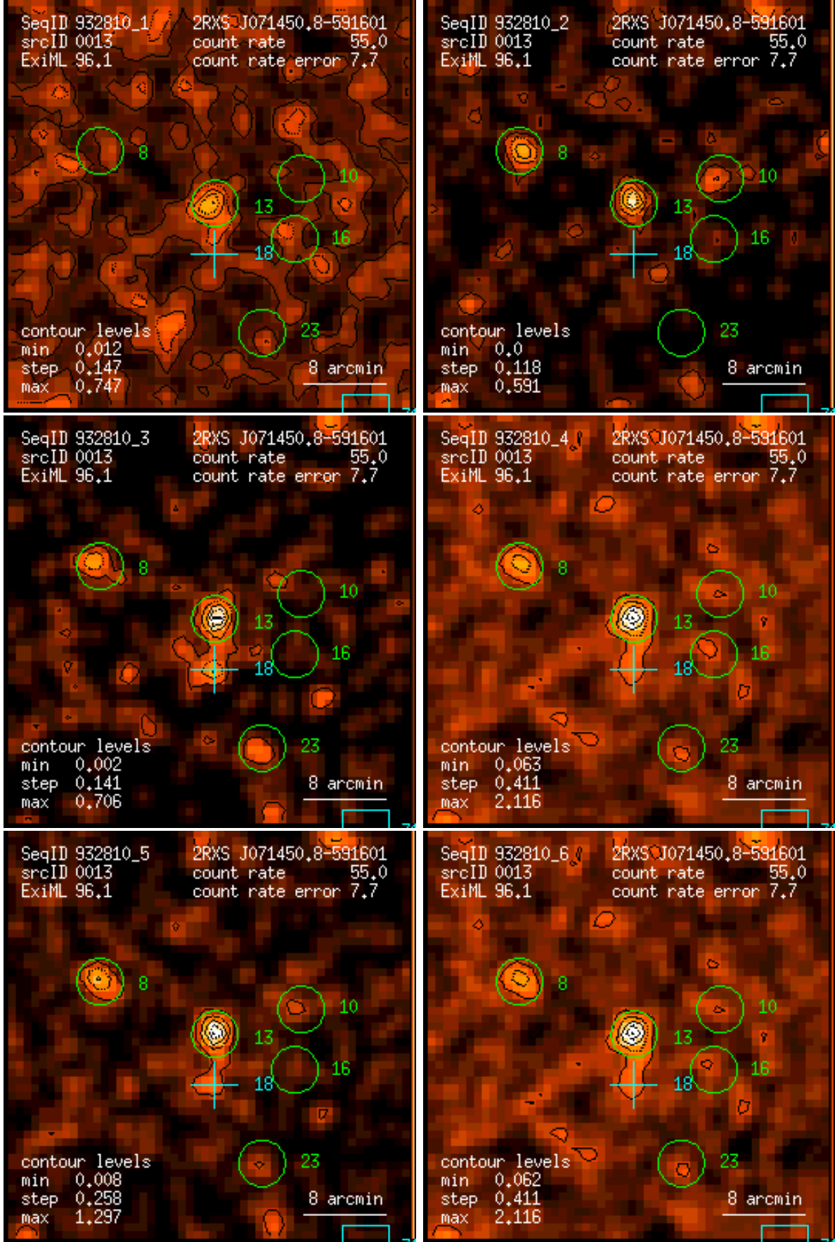
Figure 13: RASS 932810: detection 0013: band rate images, Gaussian filter: (1) PSPC channels 11 – 41, (2) 52 – 90, (3) 91 – 201, (4) 11 – 235, (5) 52 – 201, (6) 11 – 201. Broad band rates in counts/ks. Band rate contour levels in counts/ks/arcmin 2 .
