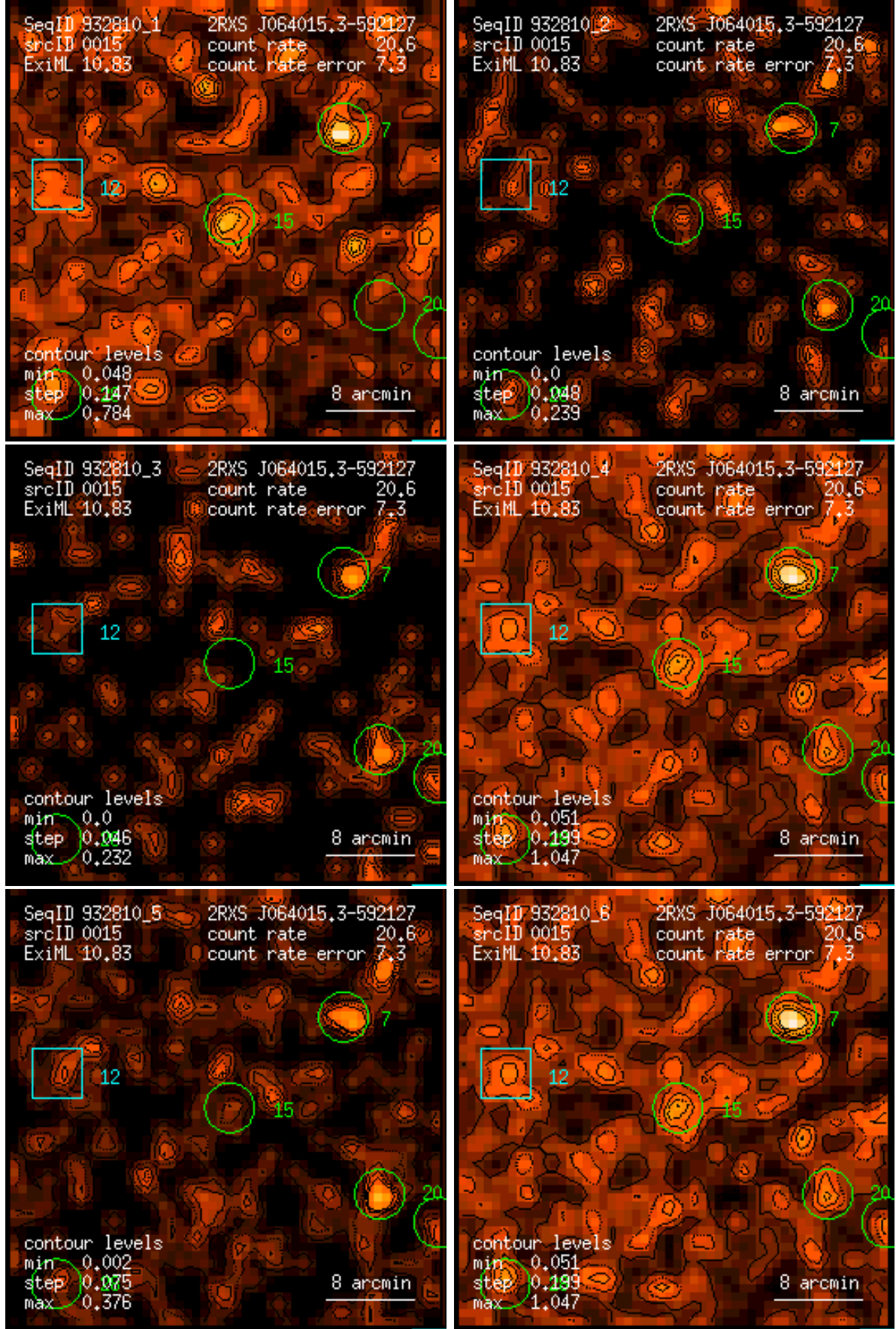
Figure 15: RASS 932810: detection 0015: band rate images, Gaussian filter: (1) PSPC channels 11 – 41, (2) 52 – 90, (3) 91 – 201, (4) 11 – 235, (5) 52 – 201, (6) 11 – 201. Broad band rates in counts/ks. Band rate contour levels in counts/ks/arcmin 2 .
