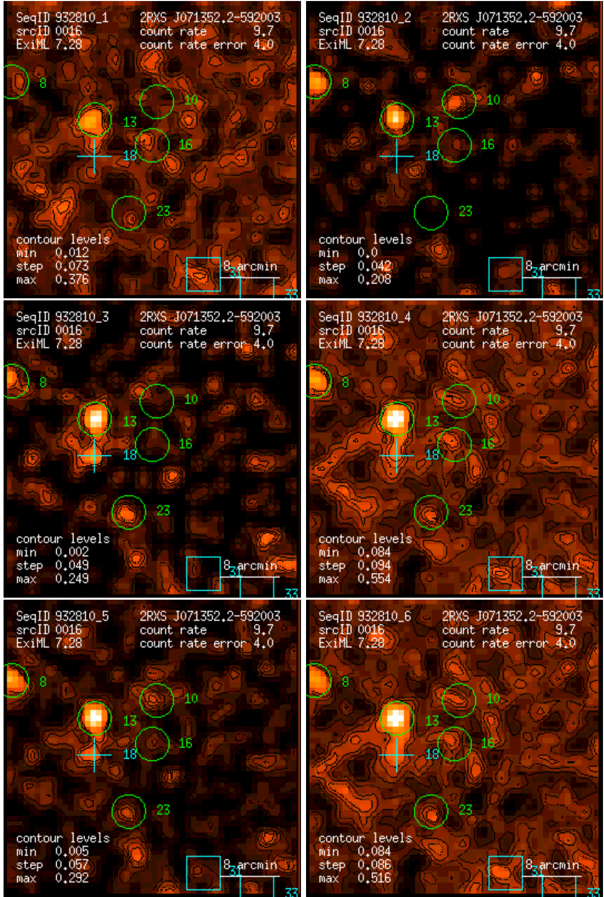
Figure 16: RASS 932810: detection 0016: band rate images, Gaussian filter: (1) PSPC channels 11 – 41, (2) 52 – 90, (3) 91 – 201, (4) 11 – 235, (5) 52 – 201, (6) 11 – 201. Broad band rates in counts/ks. Band rate contour levels in counts/ks/arcmin 2 .
