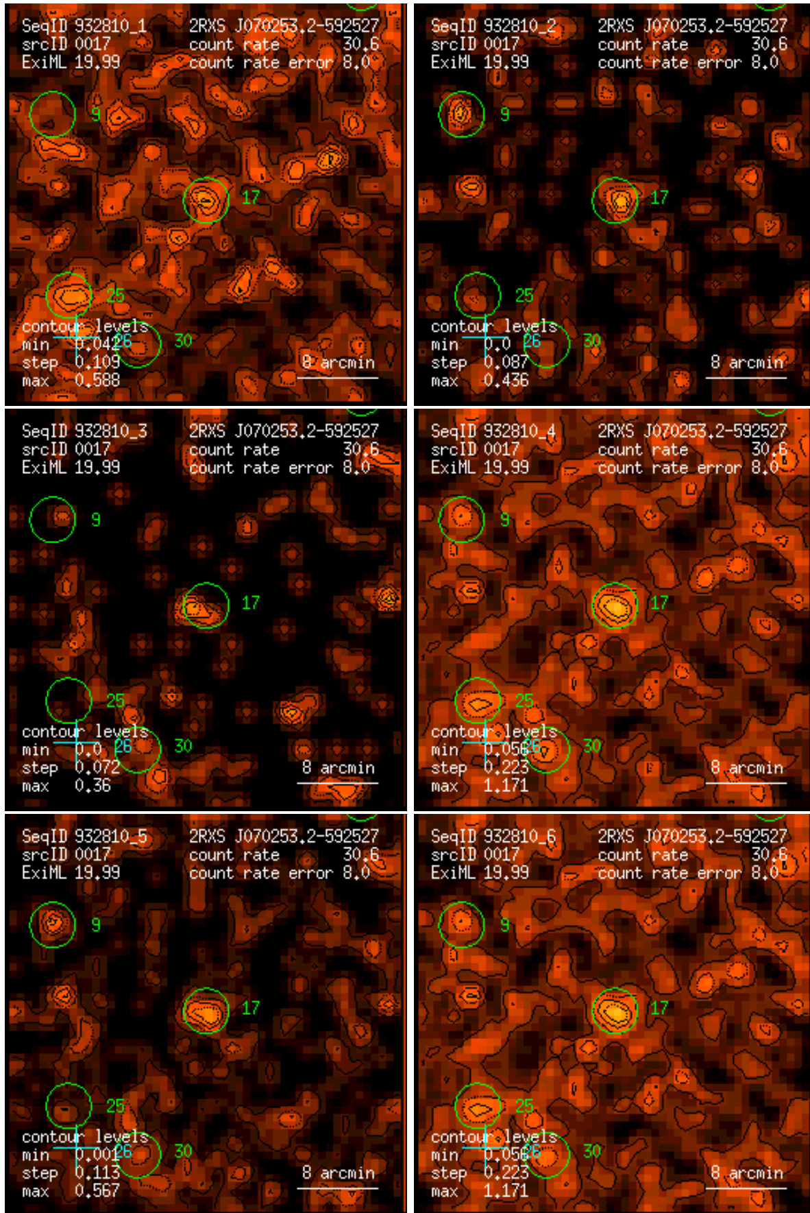
Figure 17: RASS 932810: detection 0017: band rate images, Gaussian filter: (1) PSPC channels 11 – 41, (2) 52 – 90, (3) 91 – 201, (4) 11 – 235, (5) 52 – 201, (6) 11 – 201. Broad band rates in counts/ks. Band rate contour levels in counts/ks/arcmin 2 .
