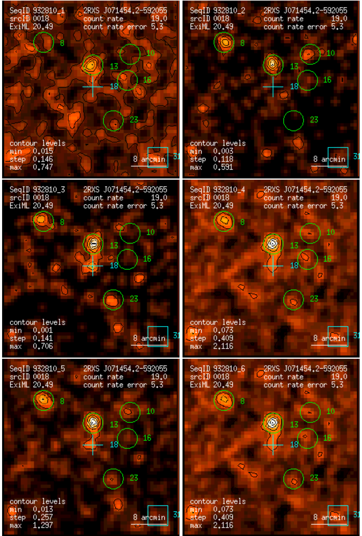
Figure 18: RASS 932810: detection 0018: band rate images, Gaussian filter: (1) PSPC channels 11 – 41, (2) 52 – 90, (3) 91 – 201, (4) 11 – 235, (5) 52 – 201, (6) 11 – 201. Broad band rates in counts/ks. Band rate contour levels in counts/ks/arcmin 2 .
