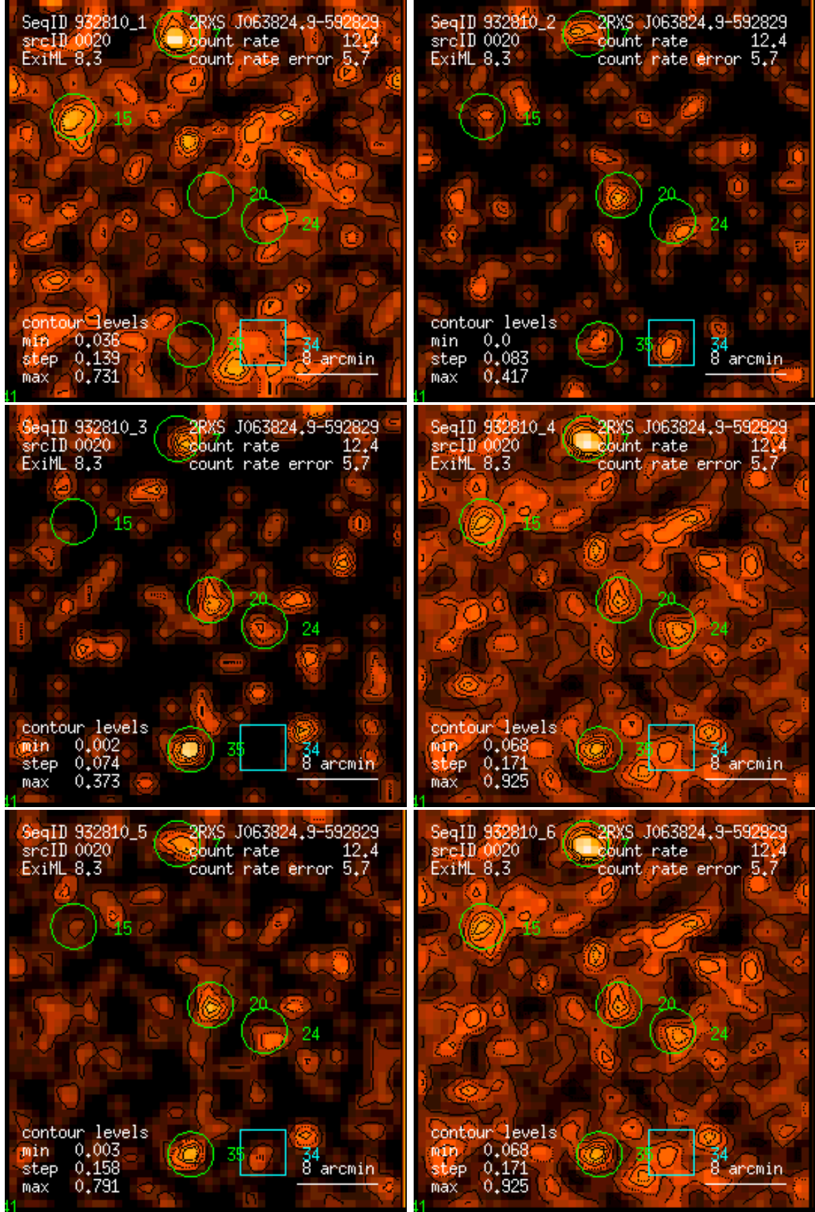
Figure 20: RASS 932810: detection 0020: band rate images, Gaussian filter: (1) PSPC channels 11 – 41, (2) 52 – 90, (3) 91 – 201, (4) 11 – 235, (5) 52 – 201, (6) 11 – 201. Broad band rates in counts/ks. Band rate contour levels in counts/ks/arcmin 2 .
