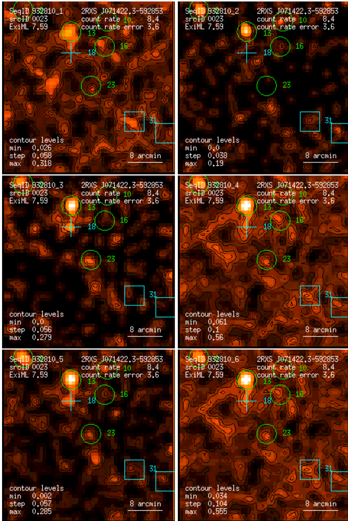
Figure 23: RASS 932810: detection 0023: band rate images, Gaussian filter: (1) PSPC channels 11 – 41, (2) 52 – 90, (3) 91 – 201, (4) 11 – 235, (5) 52 – 201, (6) 11 – 201. Broad band rates in counts/ks. Band rate contour levels in counts/ks/arcmin 2 .
