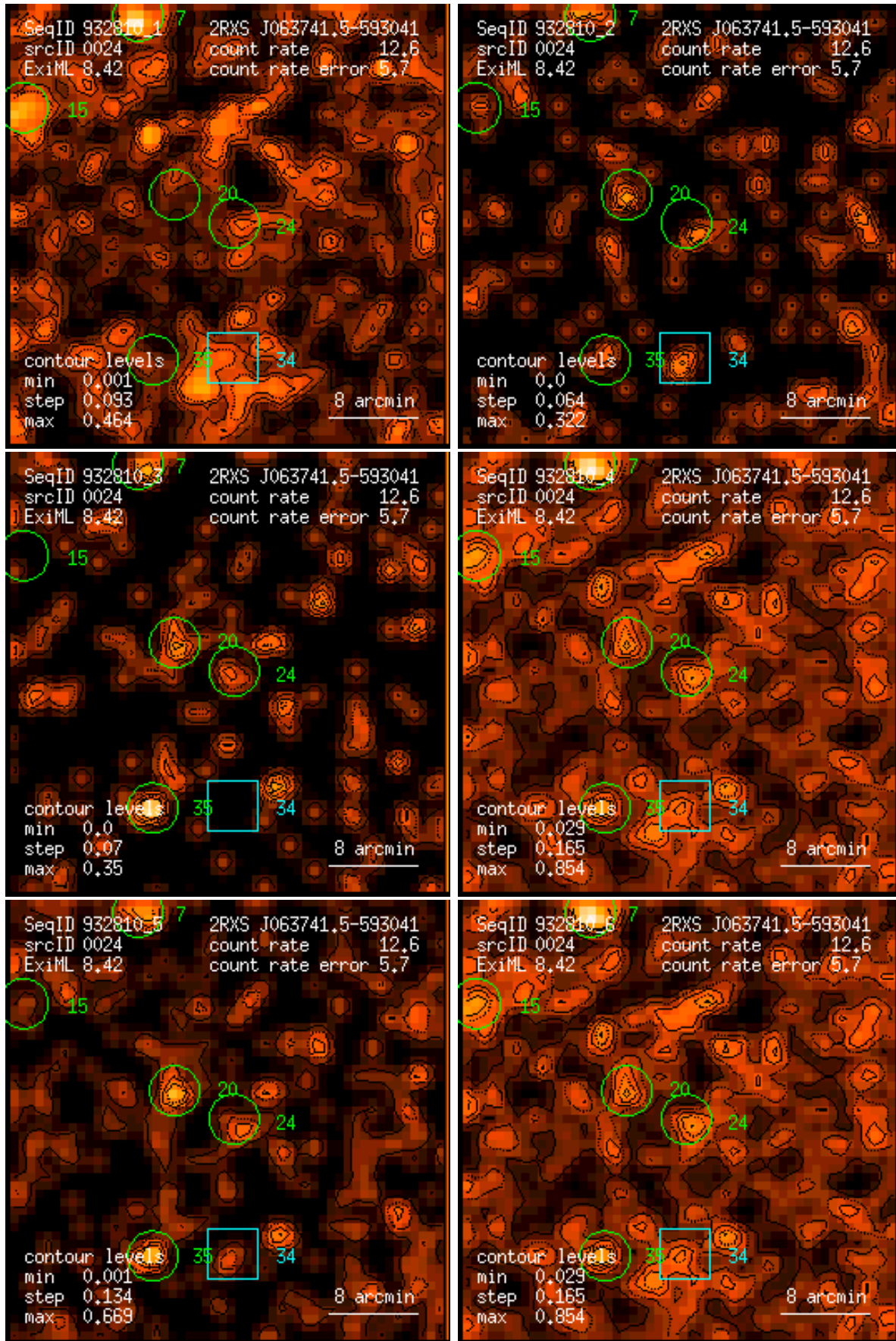
Figure 24: RASS 932810: detection 0024: band rate images, Gaussian filter: (1) PSPC channels 11 – 41, (2) 52 – 90, (3) 91 – 201, (4) 11 – 235, (5) 52 – 201, (6) 11 – 201. Broad band rates in counts/ks. Band rate contour levels in counts/ks/arcmin 2 .
