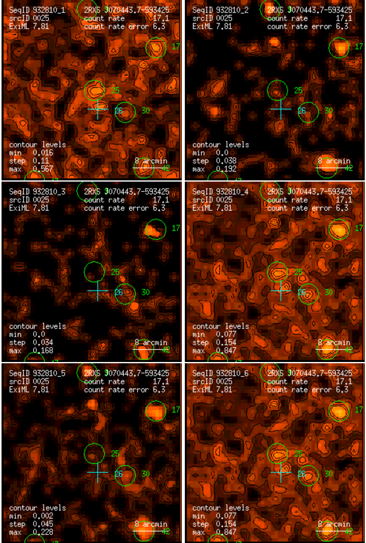
Figure 25: RASS 932810: detection 0025: band rate images, Gaussian filter: (1) PSPC channels 11 – 41, (2) 52 – 90, (3) 91 – 201, (4) 11 – 235, (5) 52 – 201, (6) 11 – 201. Broad band rates in counts/ks. Band rate contour levels in counts/ks/arcmin 2 .
