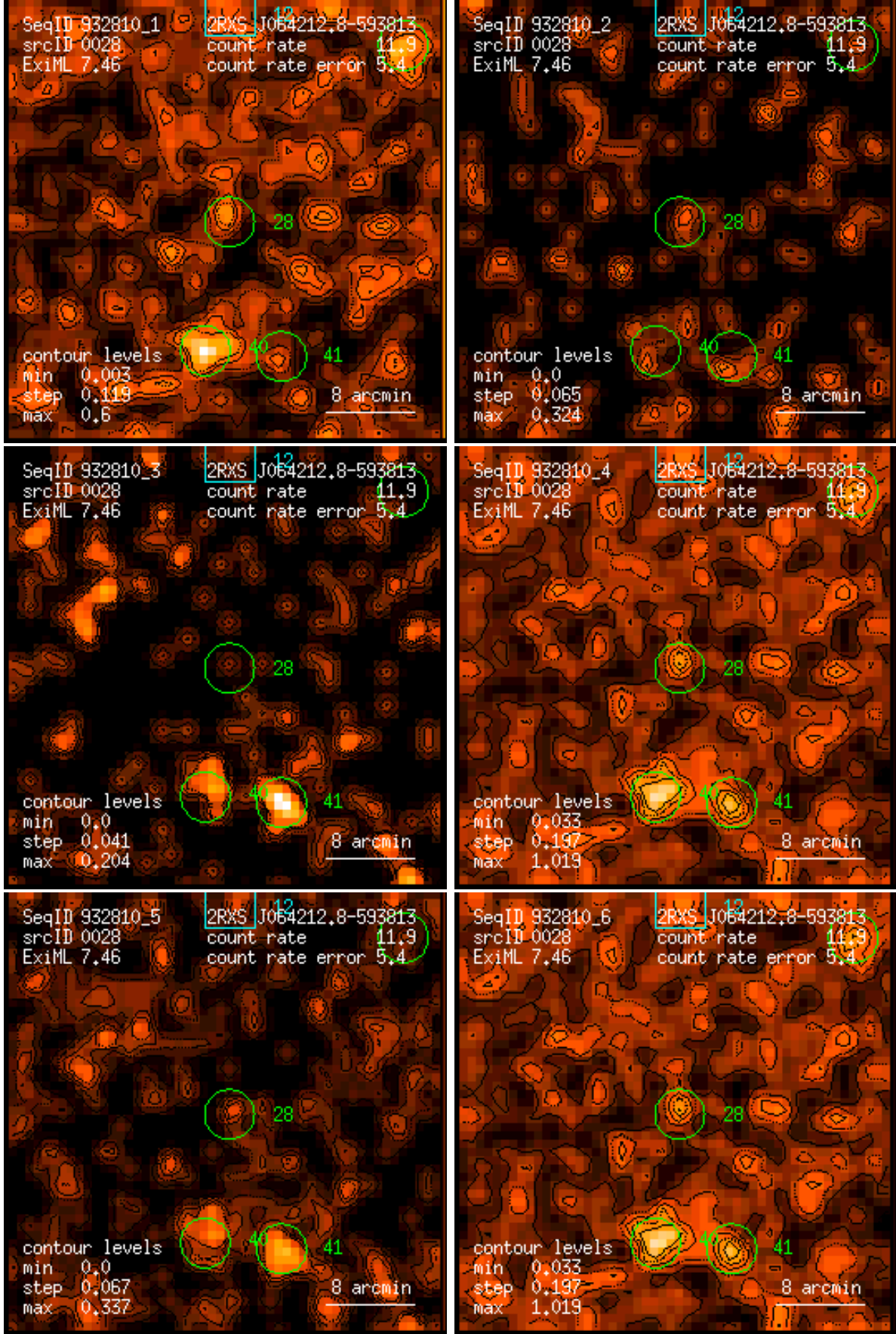
Figure 28: RASS 932810: detection 0028: band rate images, Gaussian filter: (1) PSPC channels 11 – 41, (2) 52 – 90, (3) 91 – 201, (4) 11 – 235, (5) 52 – 201, (6) 11 – 201. Broad band rates in counts/ks. Band rate contour levels in counts/ks/arcmin 2 .
