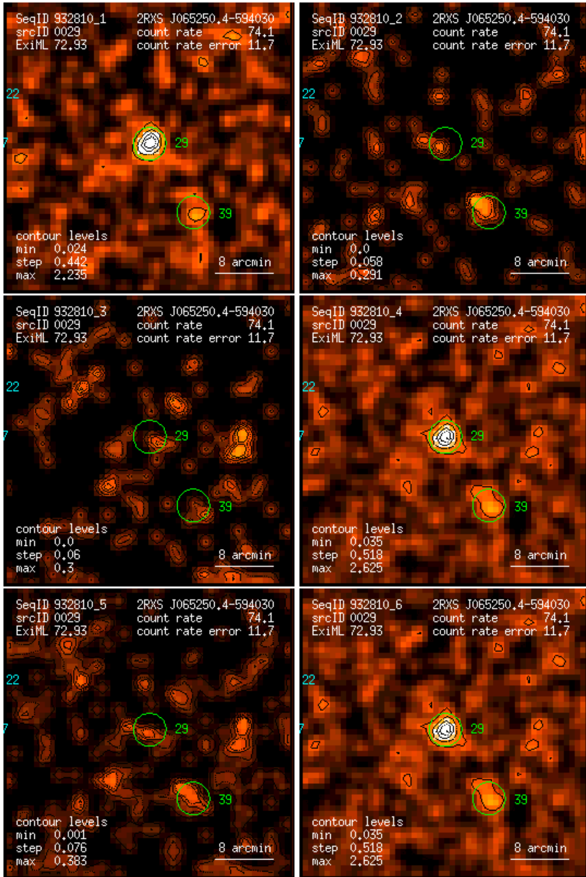
Figure 29: RASS 932810: detection 0029: band rate images, Gaussian filter: (1) PSPC channels 11 – 41, (2) 52 – 90, (3) 91 – 201, (4) 11 – 235, (5) 52 – 201, (6) 11 – 201. Broad band rates in counts/ks. Band rate contour levels in counts/ks/arcmin 2 .
