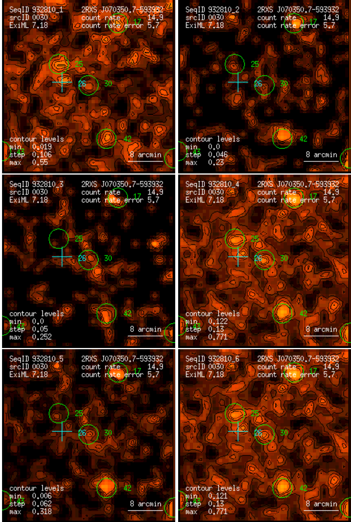
Figure 30: RASS 932810: detection 0030: band rate images, Gaussian filter: (1) PSPC channels 11 – 41, (2) 52 – 90, (3) 91 – 201, (4) 11 – 235, (5) 52 – 201, (6) 11 – 201. Broad band rates in counts/ks. Band rate contour levels in counts/ks/arcmin 2 .
