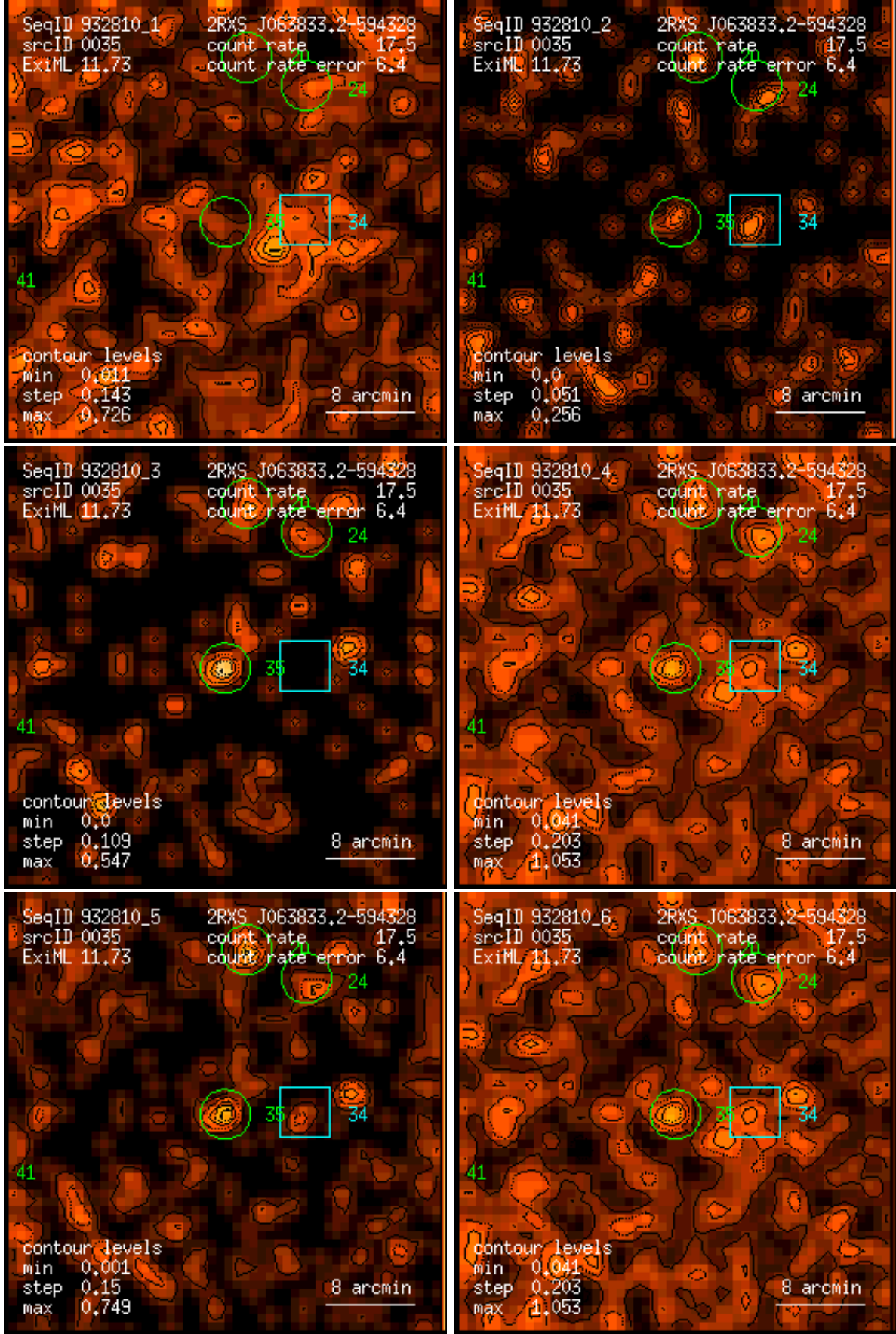
Figure 35: RASS 932810: detection 0035: band rate images, Gaussian filter: (1) PSPC channels 11 – 41, (2) 52 – 90, (3) 91 – 201, (4) 11 – 235, (5) 52 – 201, (6) 11 – 201. Broad band rates in counts/ks. Band rate contour levels in counts/ks/arcmin 2 .
