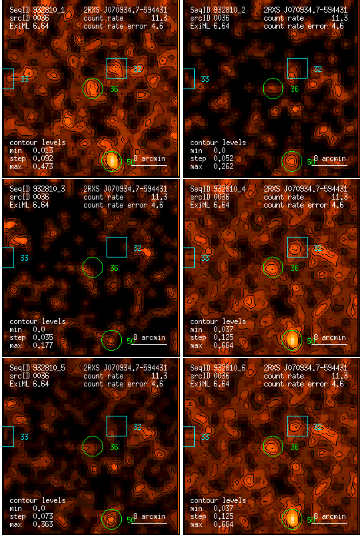
Figure 36: RASS 932810: detection 0036: band rate images, Gaussian filter: (1) PSPC channels 11 – 41, (2) 52 – 90, (3) 91 – 201, (4) 11 – 235, (5) 52 – 201, (6) 11 – 201. Broad band rates in counts/ks. Band rate contour levels in counts/ks/arcmin 2 .
