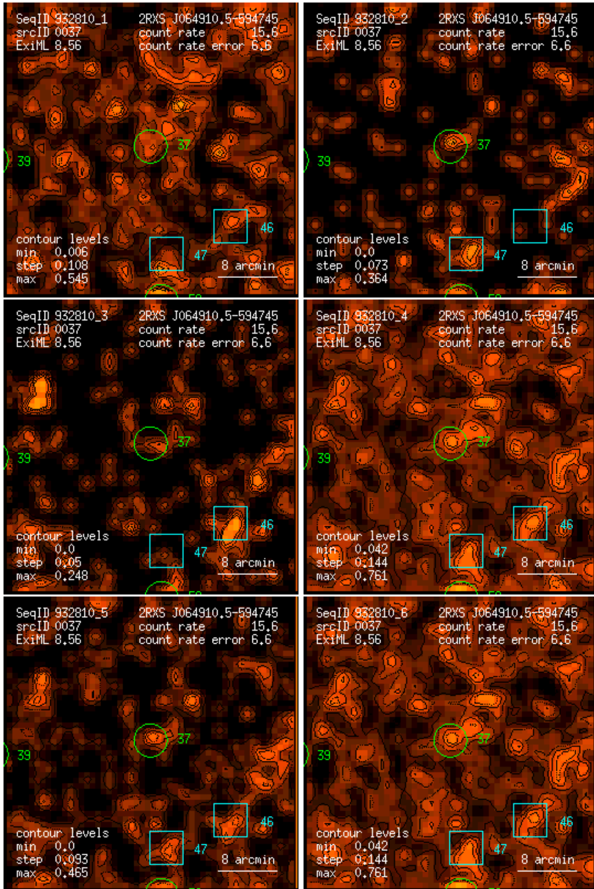
Figure 37: RASS 932810: detection 0037: band rate images, Gaussian filter: (1) PSPC channels 11 – 41, (2) 52 – 90, (3) 91 – 201, (4) 11 – 235, (5) 52 – 201, (6) 11 – 201. Broad band rates in counts/ks. Band rate contour levels in counts/ks/arcmin 2 .
