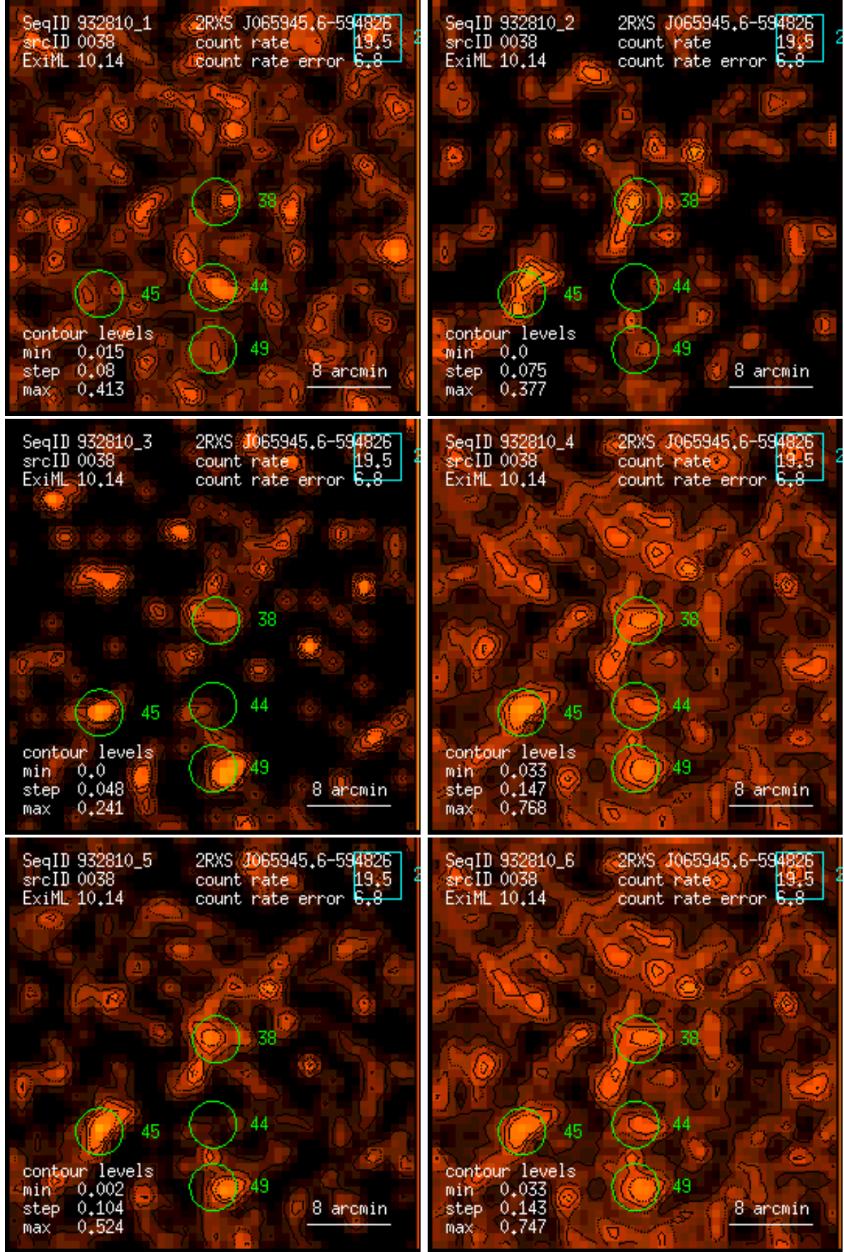
Figure 38: RASS 932810: detection 0038: band rate images, Gaussian filter: (1) PSPC channels 11 – 41, (2) 52 – 90, (3) 91 – 201, (4) 11 – 235, (5) 52 – 201, (6) 11 – 201. Broad band rates in counts/ks. Band rate contour levels in counts/ks/arcmin 2 .
