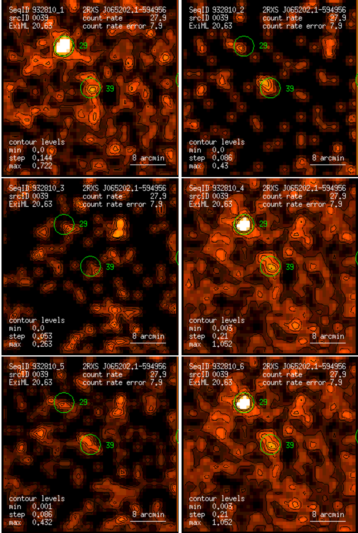
Figure 39: RASS 932810: detection 0039: band rate images, Gaussian filter: (1) PSPC channels 11 – 41, (2) 52 – 90, (3) 91 – 201, (4) 11 – 235, (5) 52 – 201, (6) 11 – 201. Broad band rates in counts/ks. Band rate contour levels in counts/ks/arcmin 2 .
